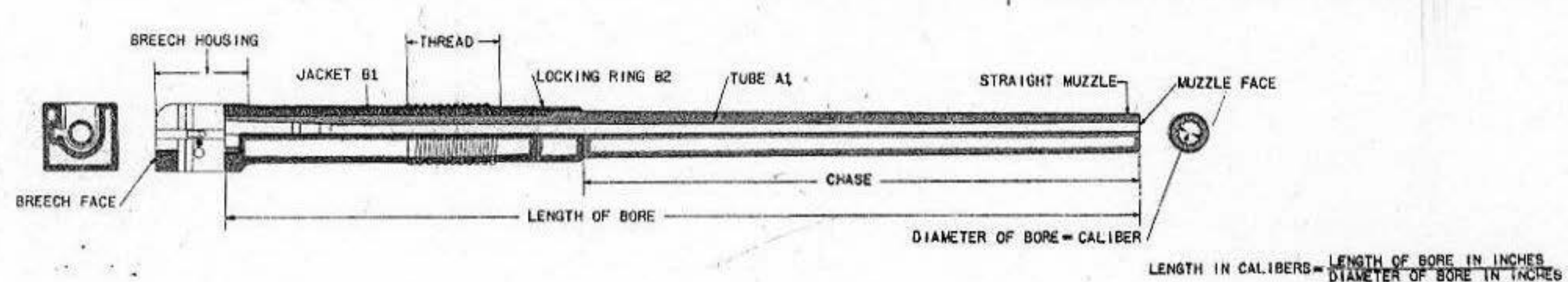
GUN NOMENCLATURE.
