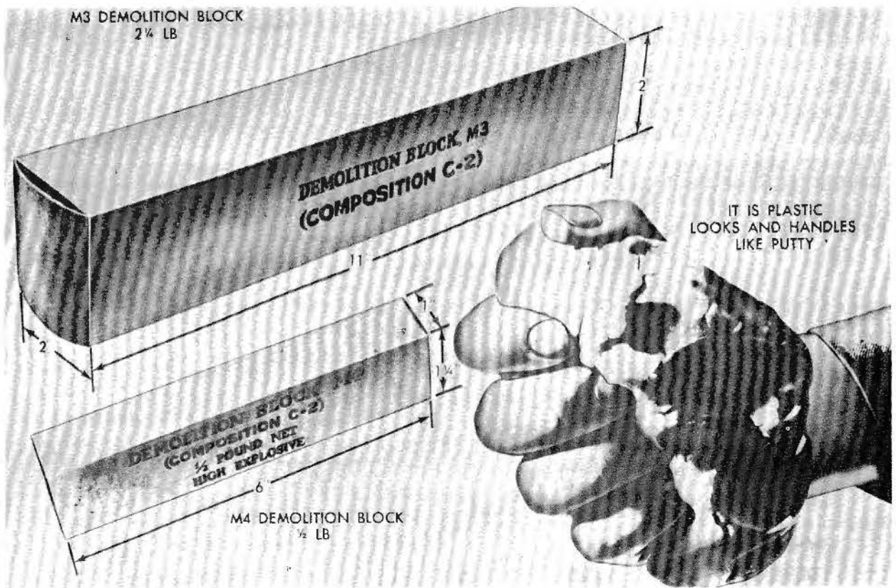
Figure 10—Demolition Blocks M3 and M4.
