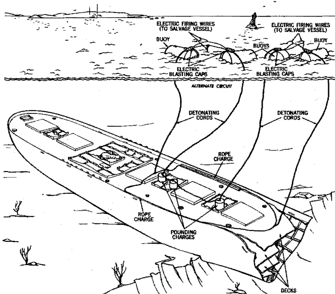
Figure 92—Ship Flattening—Flattening the Hull, Second Stage. Preparation.
