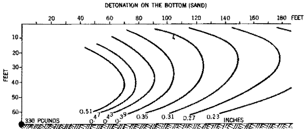
Figure 9—Equal Pressure Zones.
