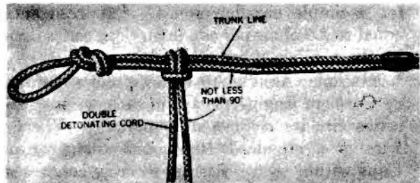
Figure 33—Girth Hitch Used to Connect Branch Line to Trunk Line of Detonating Cord.
