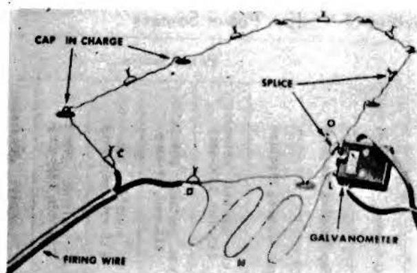
Figure 31—Locating Breaks in Firing Circuit.
