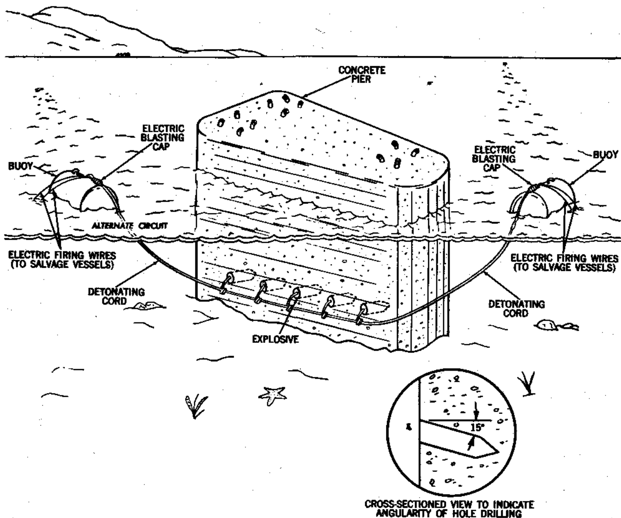
Figure 58—Dispersing a Concrete Pier with Internal Charges.
