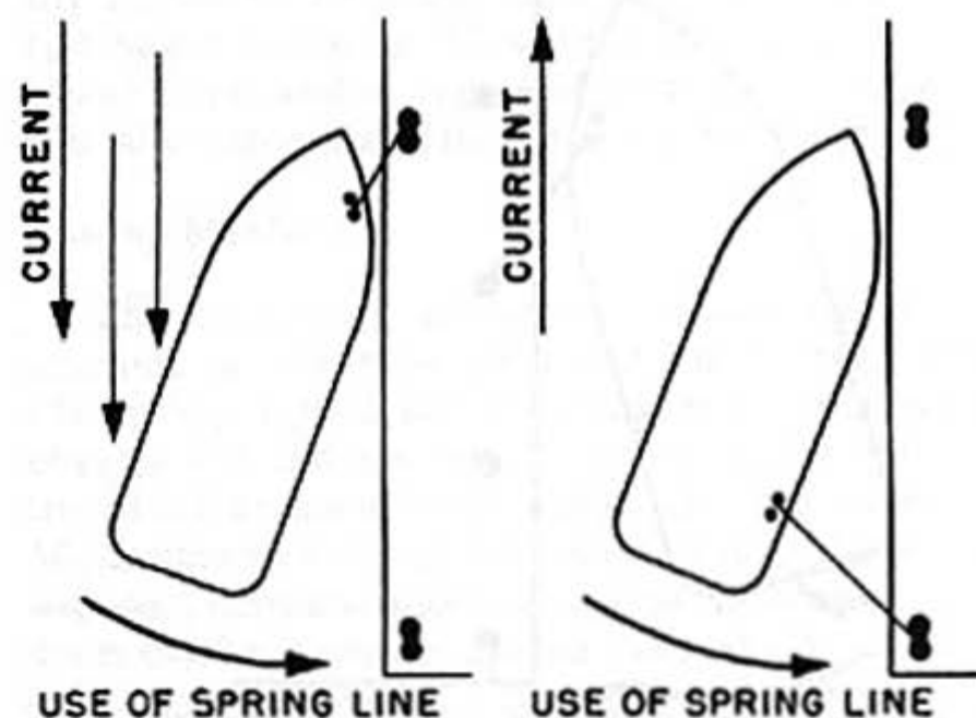
Figure 6-7.—Making use of current.
