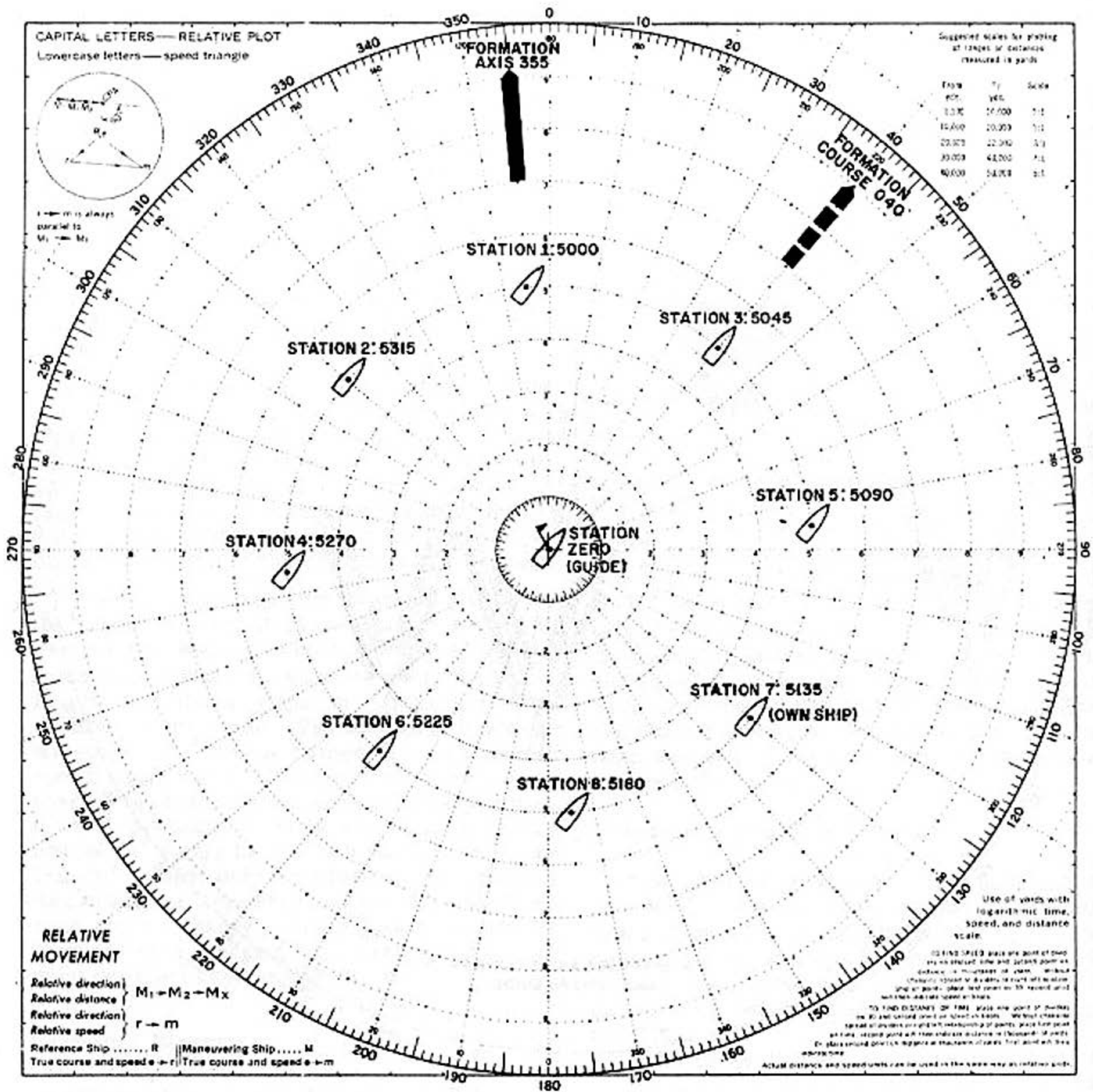
Figure 6-2.—Formation plotted on a maneuvering board.
