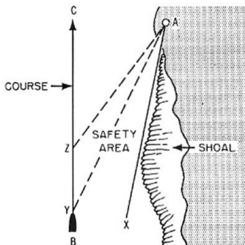
58.82 Figure 3-7.—Danger bearing.
