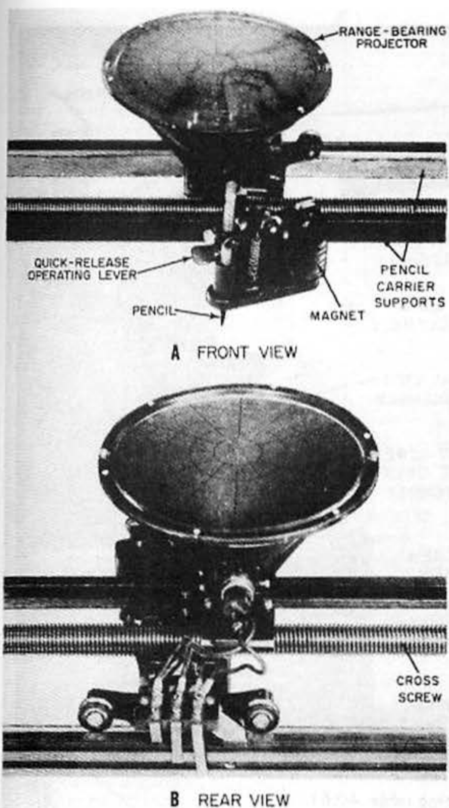
Figure 3-12. DR tracer. 40.62
