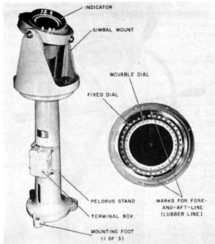
Figure 2-14. Gyro repeater. 51.131
