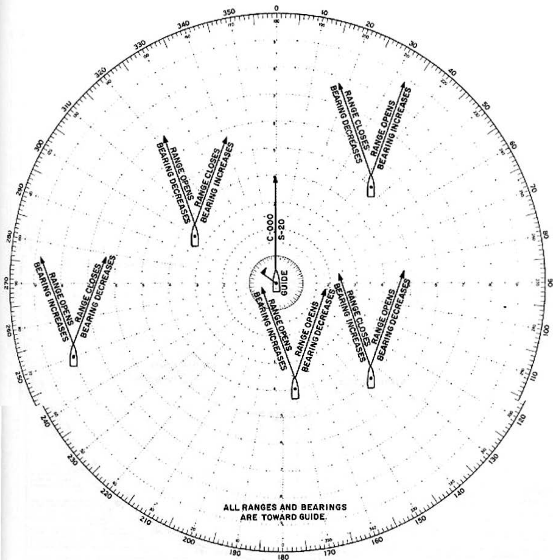
Figure 6-1.—Result of course change in station keeping.
