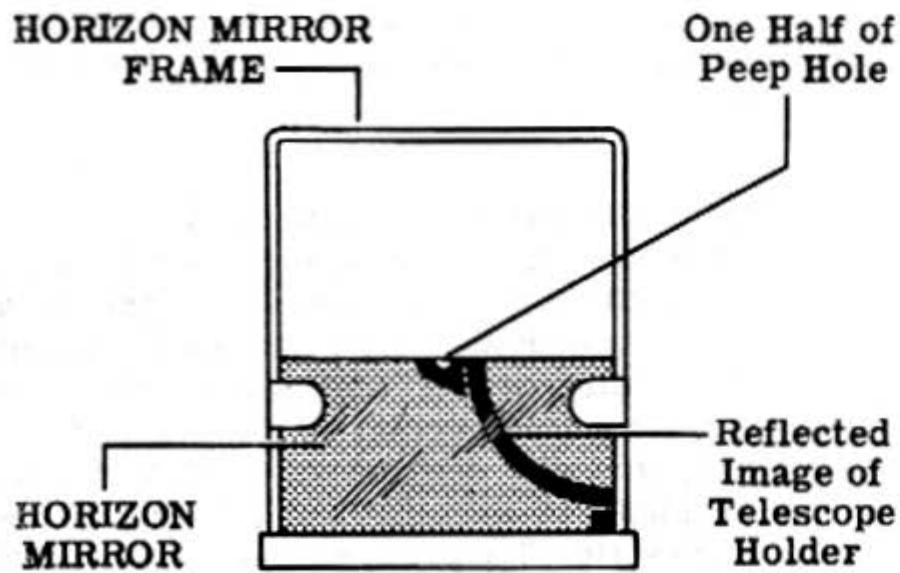
Figure 7-6.—Perpendicular adjustment of the horizon mirror.
