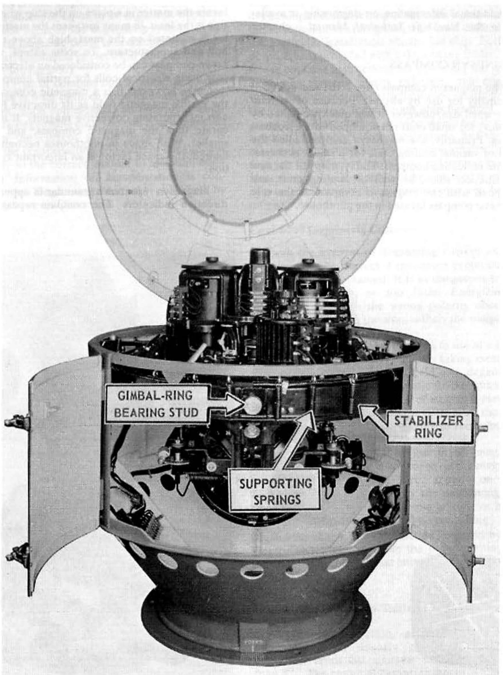
Figure 2-11. Sperry gyrocompass Mk 11 Mod 6.
