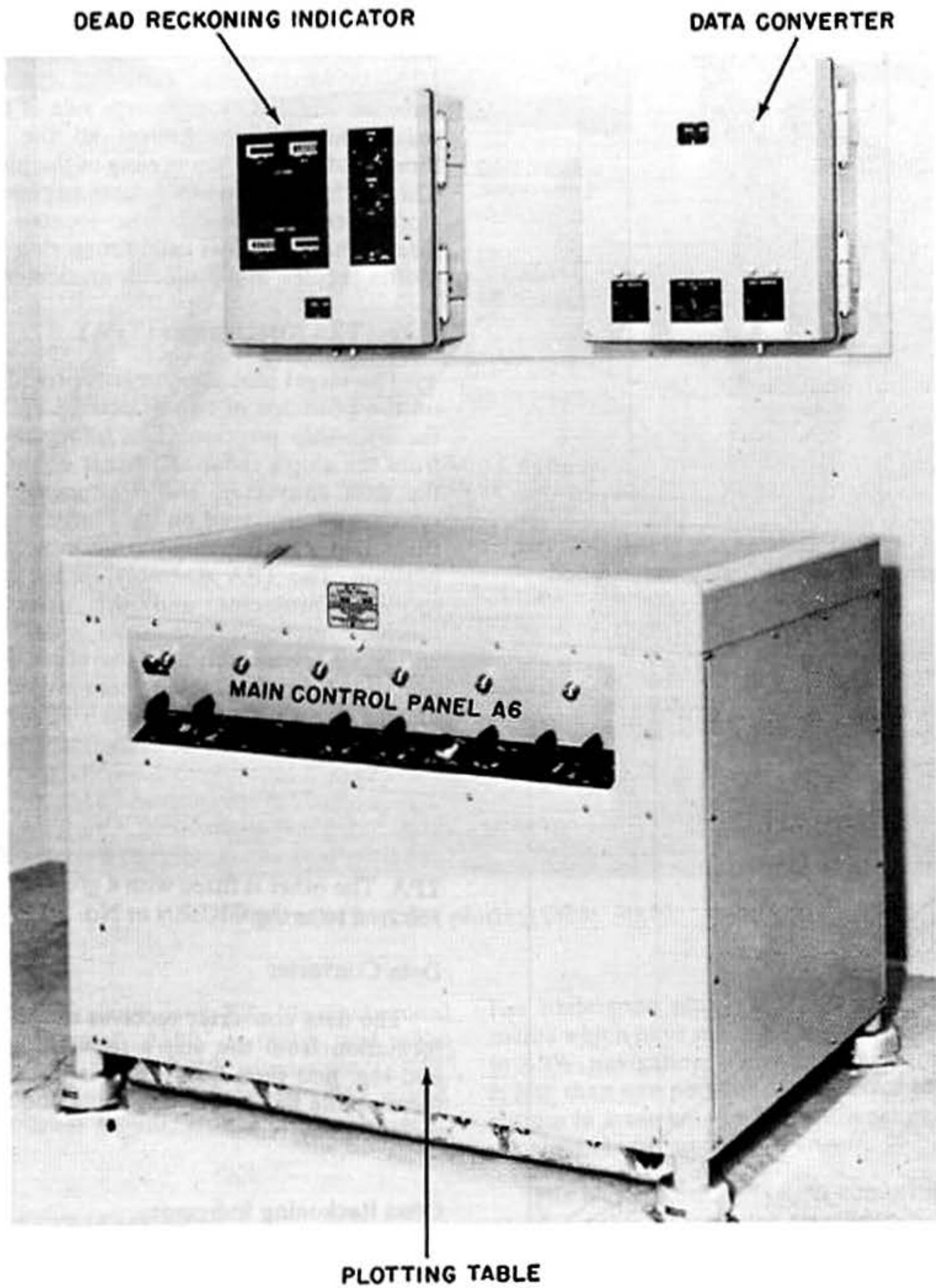
Figure 3-16. Plotting system USN Mk NC-2.
