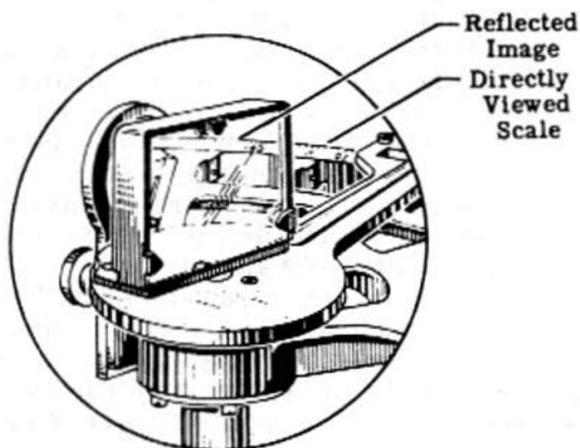
C. Index Mirror perpendicular to the plane of the Sextant Frame (Reflected image level with directly viewed scale)
