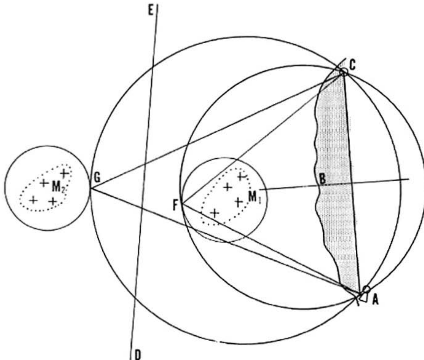
Figure 3-8.— Danger angles.
