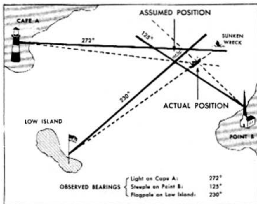
Figure A-7.—Determining compass error by adjusting bearings.
