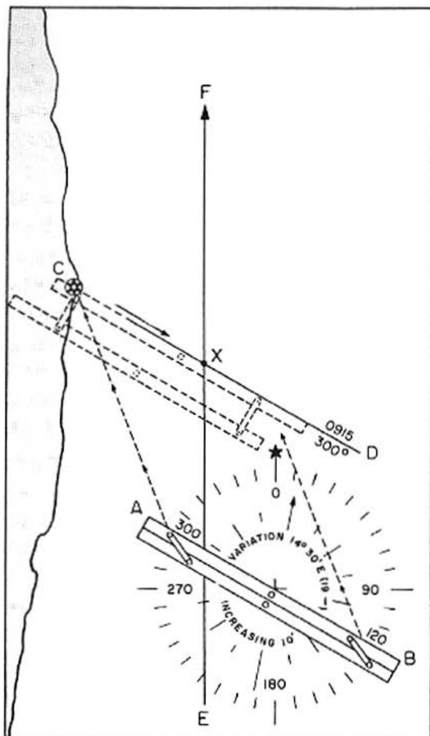
Figure 3-2.—Plotting bearings.
