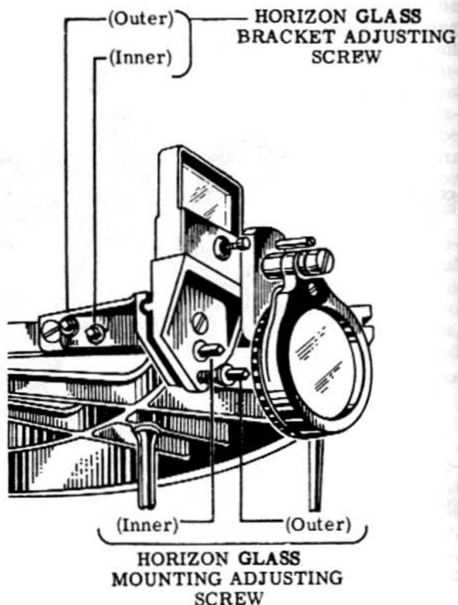
Figure 7-4.—Horizon glass mounting and adjusting screws.
