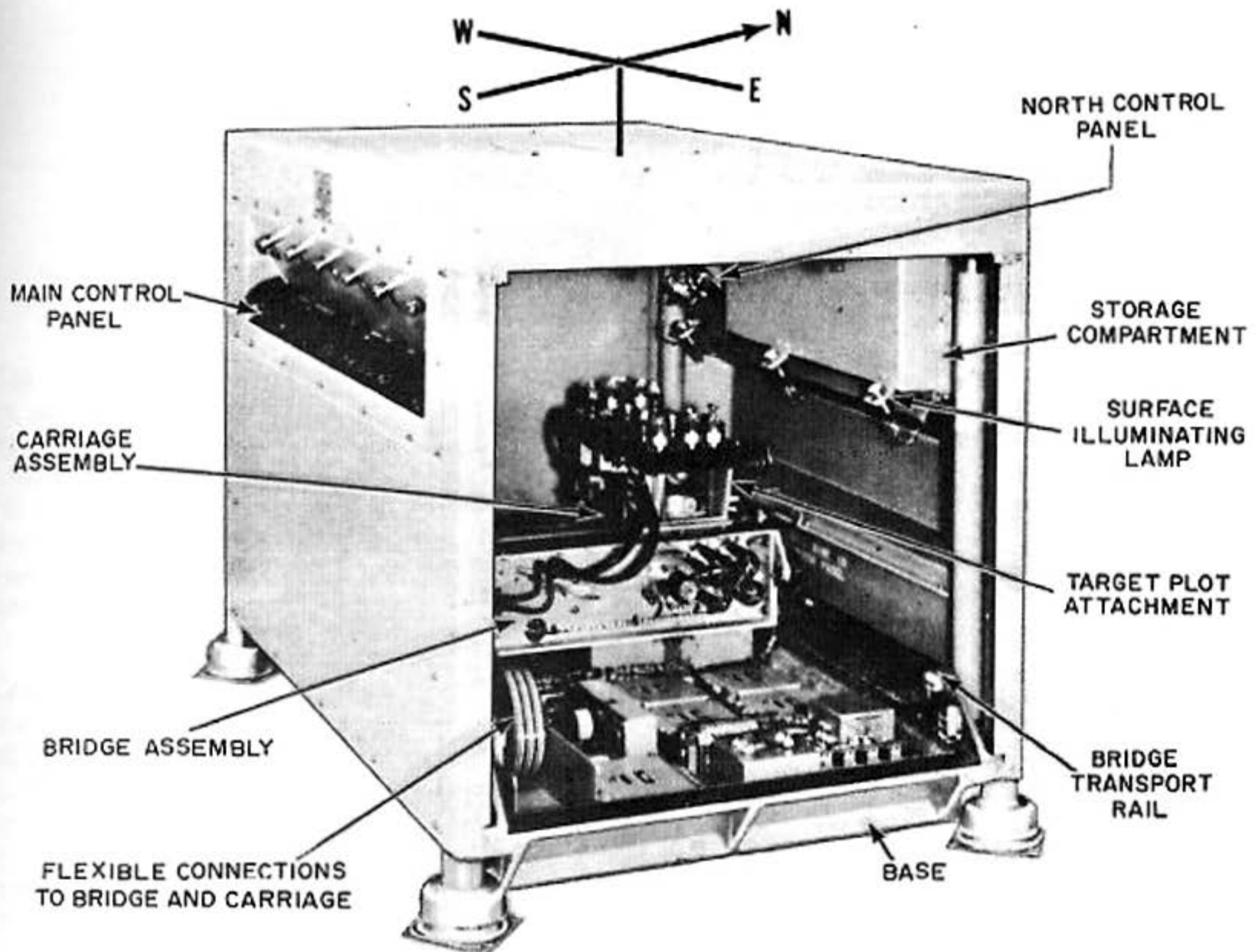
Figure 3-17. Plotting table Mk NC-2.
