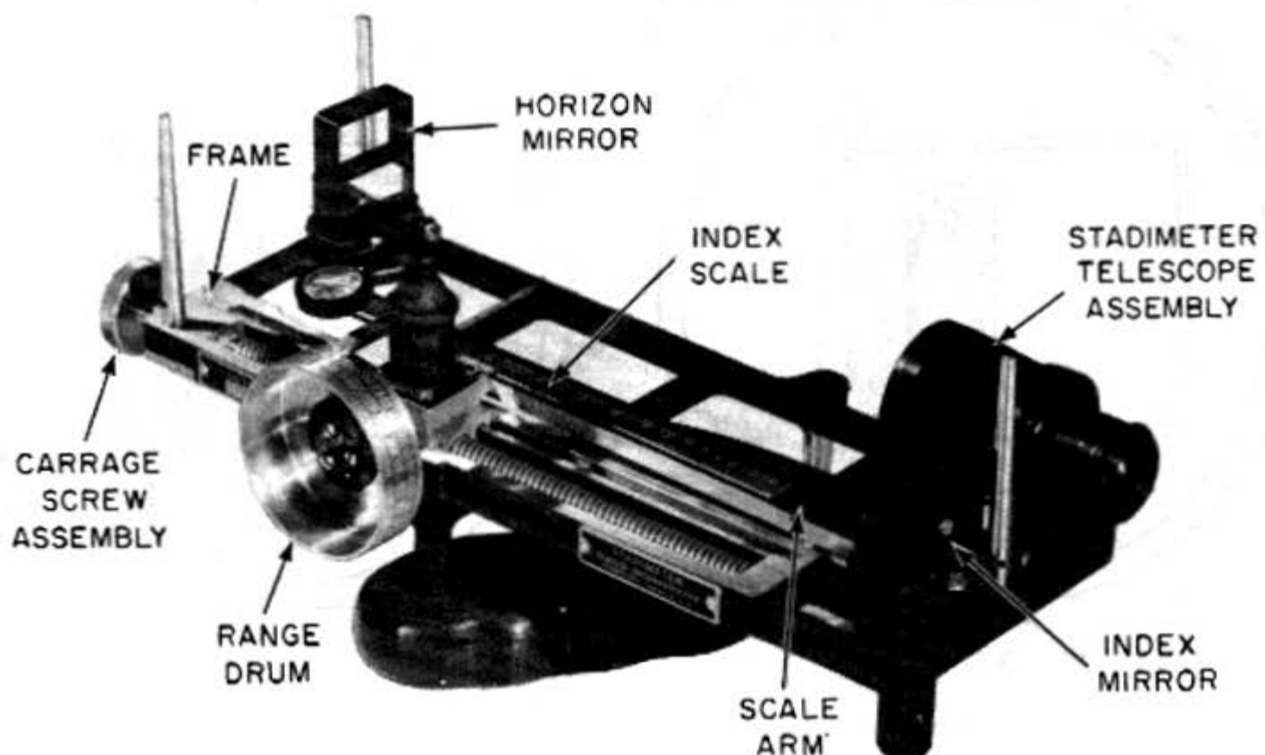
Figure 7-5. Type II Fiske stadimeter.
