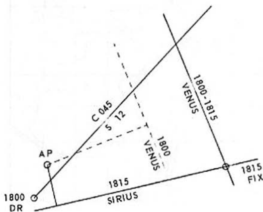
Figure 5-14.—A fix by advancing an LOP. 112.28
