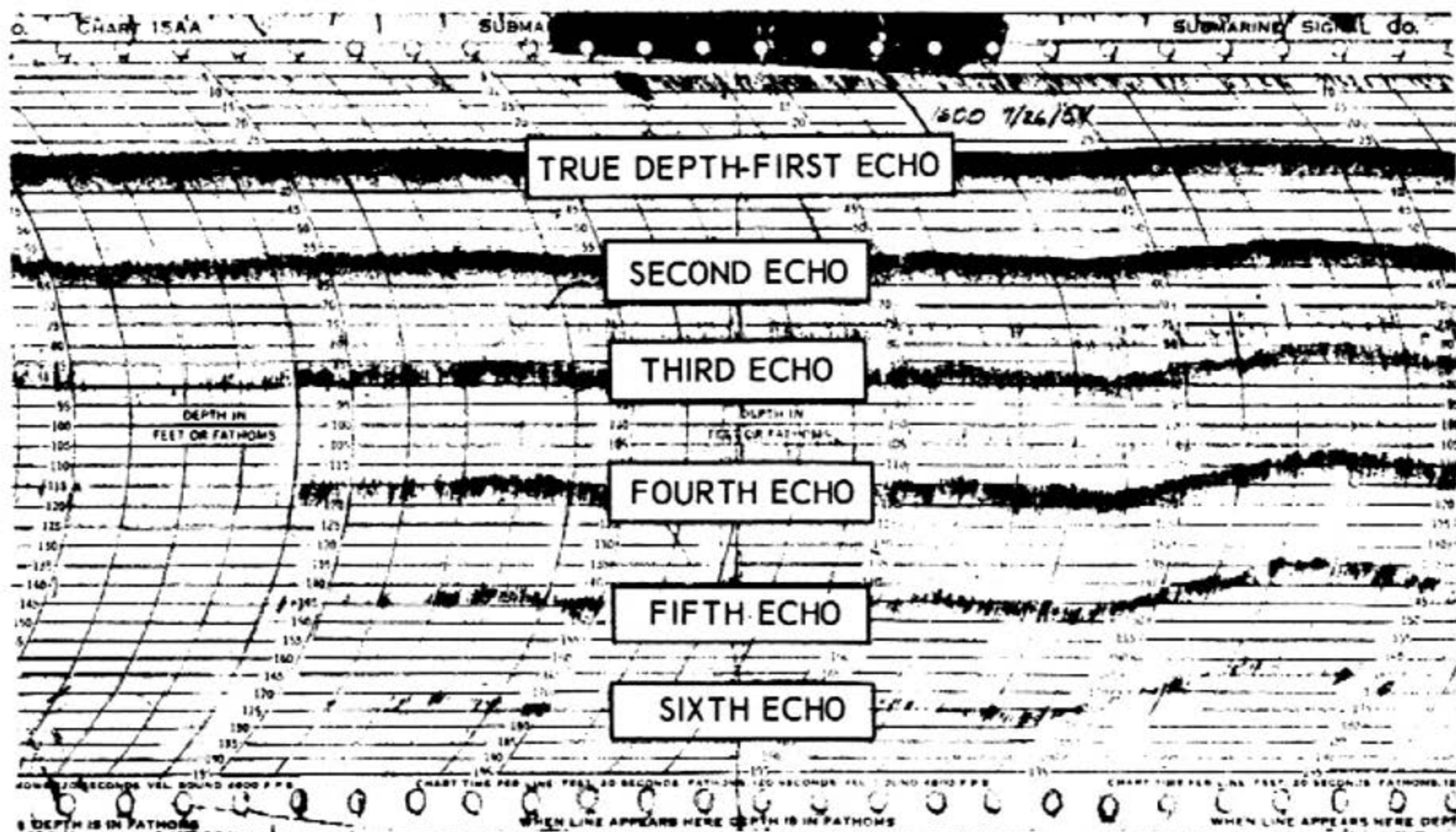
Figure 10-4.—Echogram showing multiple returns.
