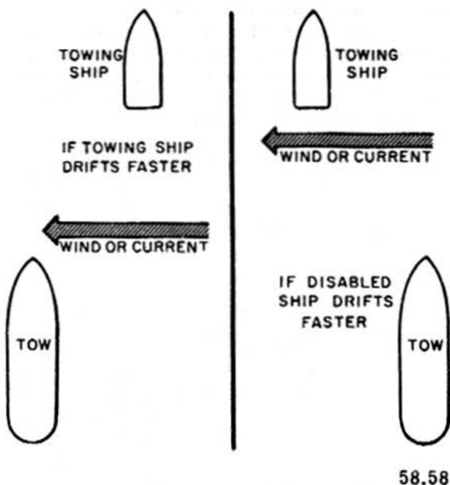
Figure 6-9.—Using drift to gain time while connecting towline.
