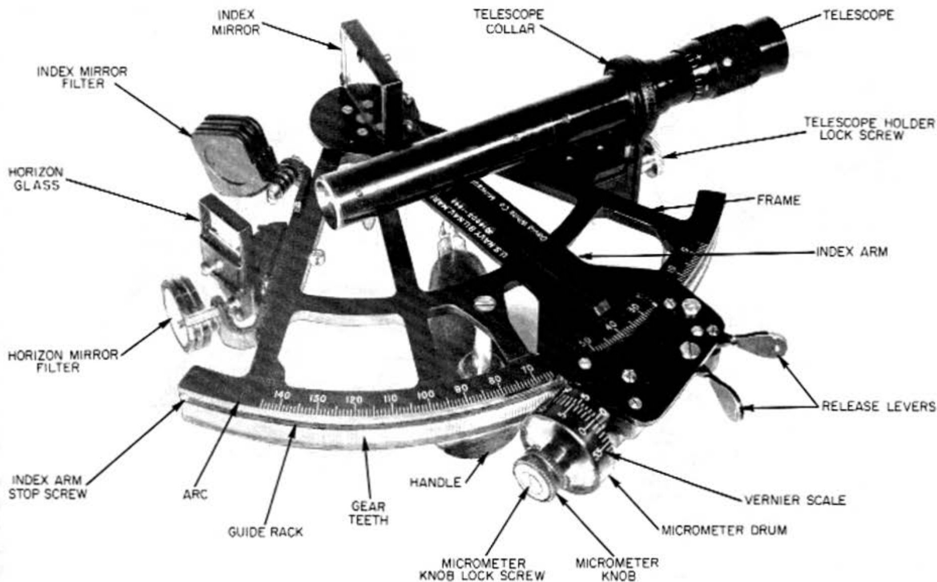
Figure 7-2. Endless tangent screw sextant. 29.268
