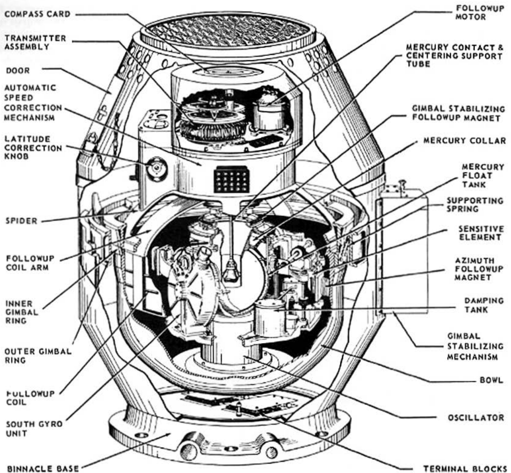
Figure 2-12.—Arma gyrocompass.
