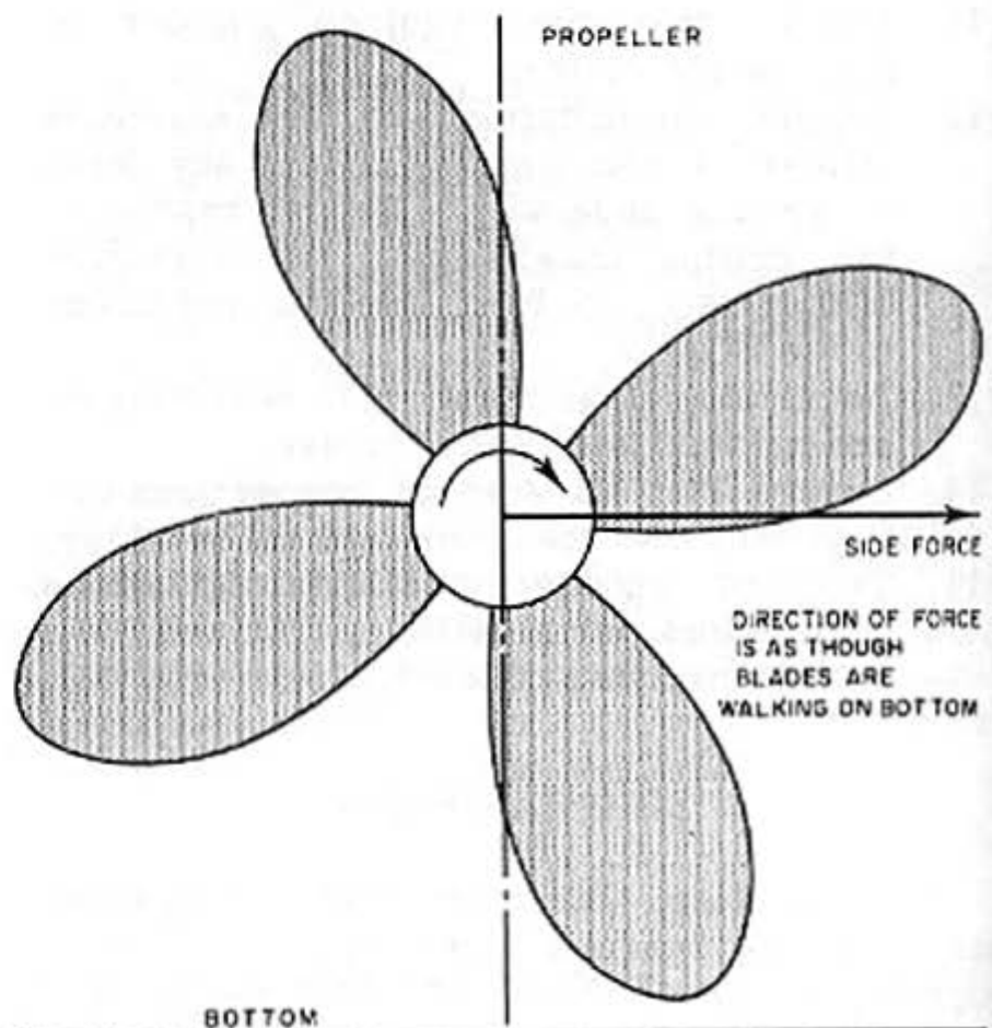
Figure 6-4.—Side force.
