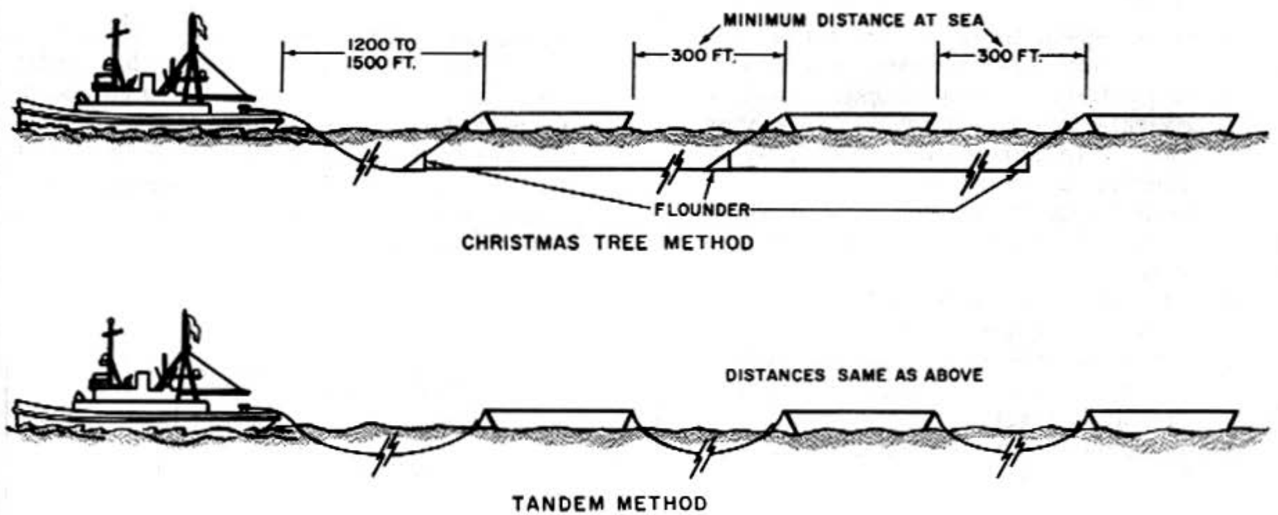
Figure 6-13.—Towing barges astern.
