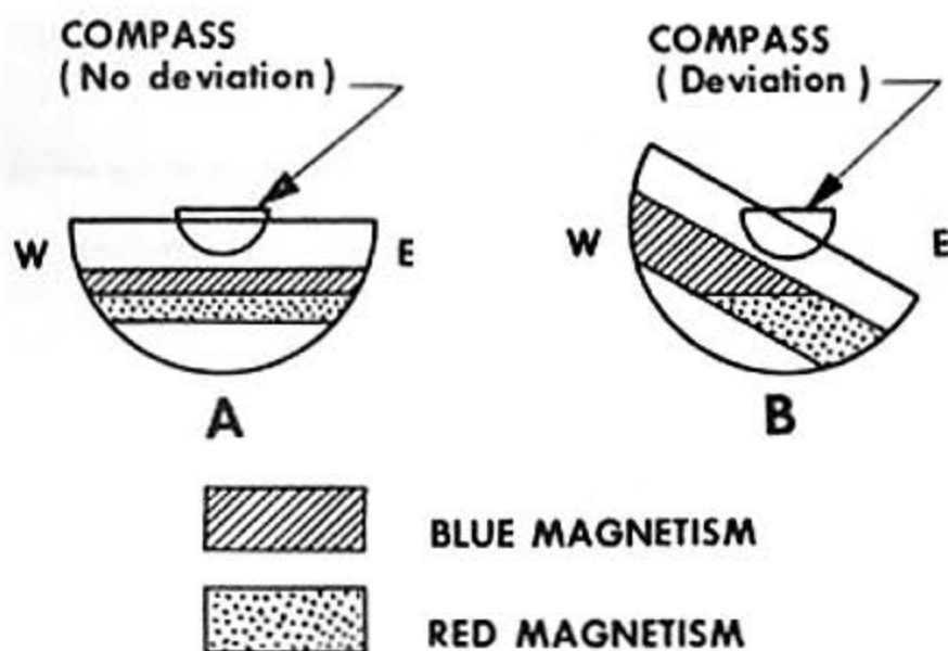
Figure 2-6.—Heeling error.
