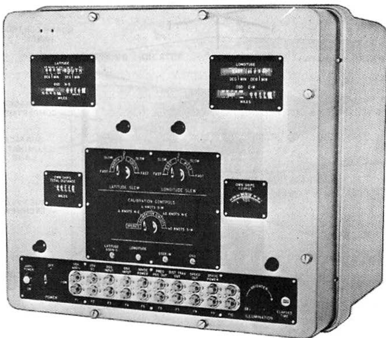
Figure 3-18. Dead reckoning analyzer-indicator Mark 9 Mod 0.
