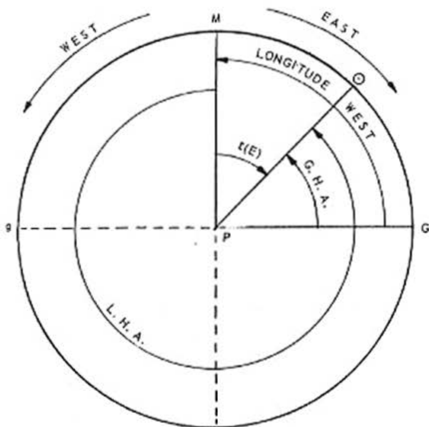
Figure 5-21.—The LHA observed from west longitude.
