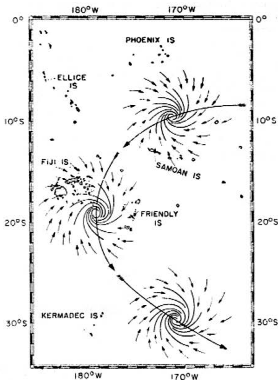
Figure 9-4. Track of a tropical cyclone originating in the Southern Hemisphere of the Central Pacific.
