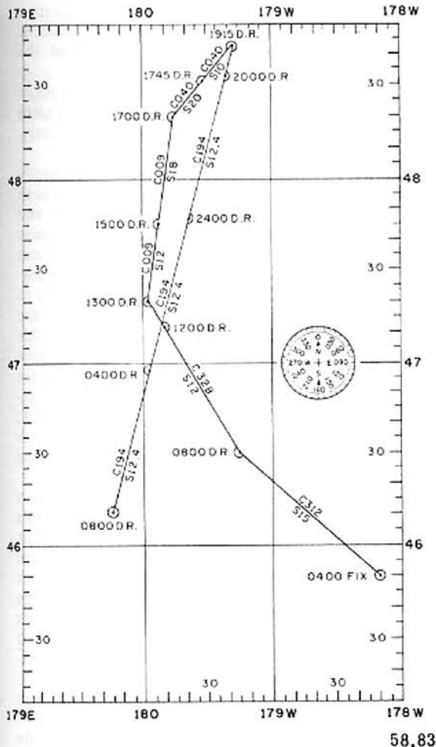
Figure 3-9.—Plotting DR position.
