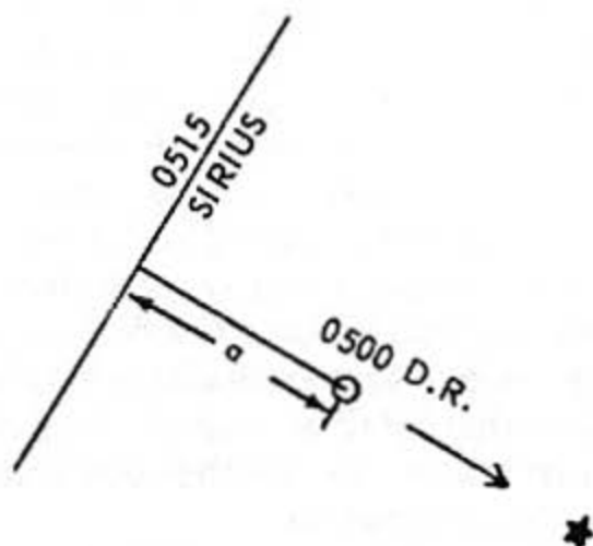
Figure 5-11.—Plotting a star LOP. 112.25
