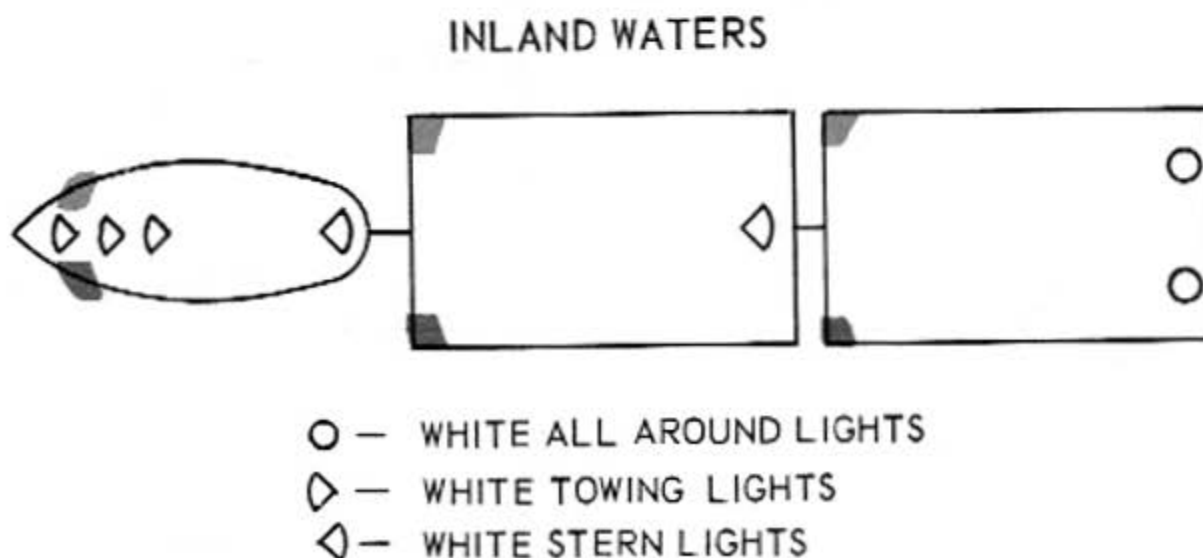
Figure 8-5. A tow in tandem. C80.121
