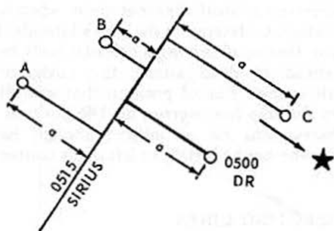
Figure 5-12.—An LOP from several APs. 112.26
