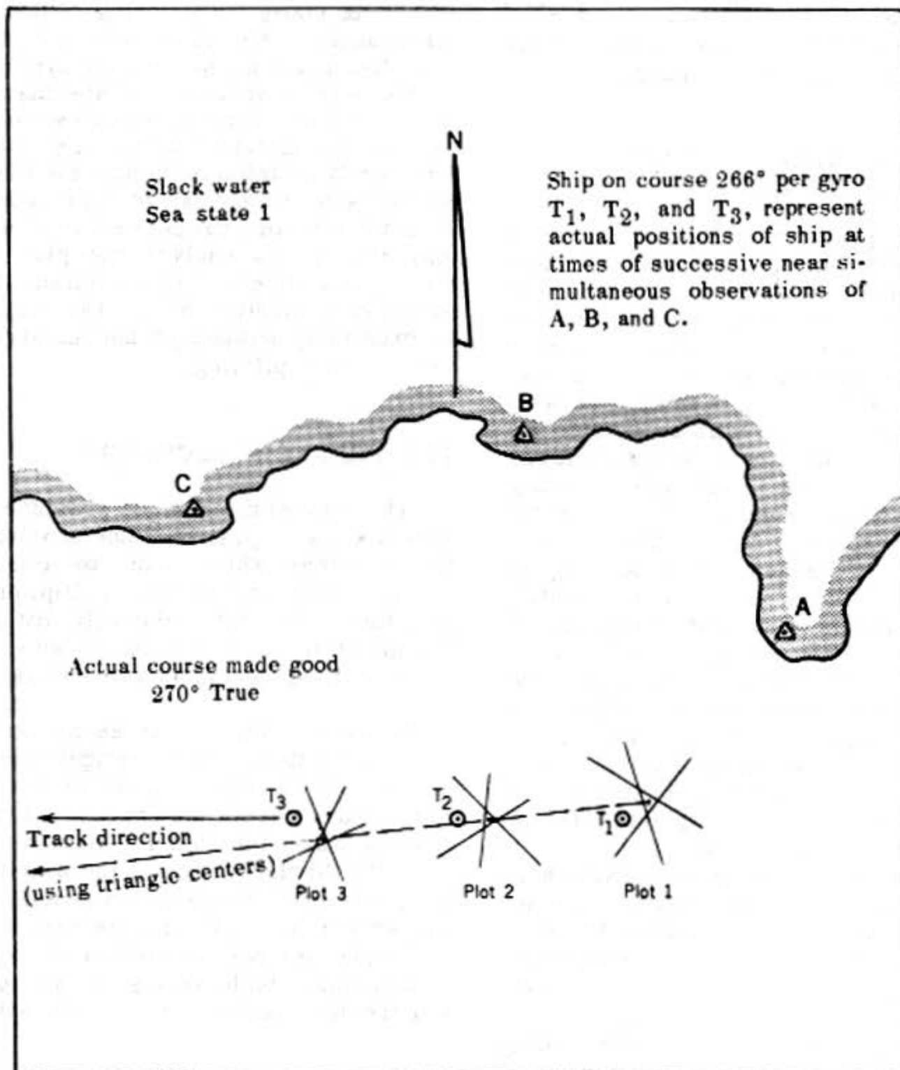
Figure A-8. Unknown compass error triangles.
