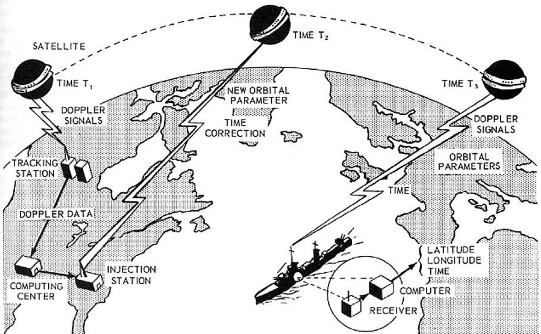
Figure 4-5. Navigational satellite system. 69.55
