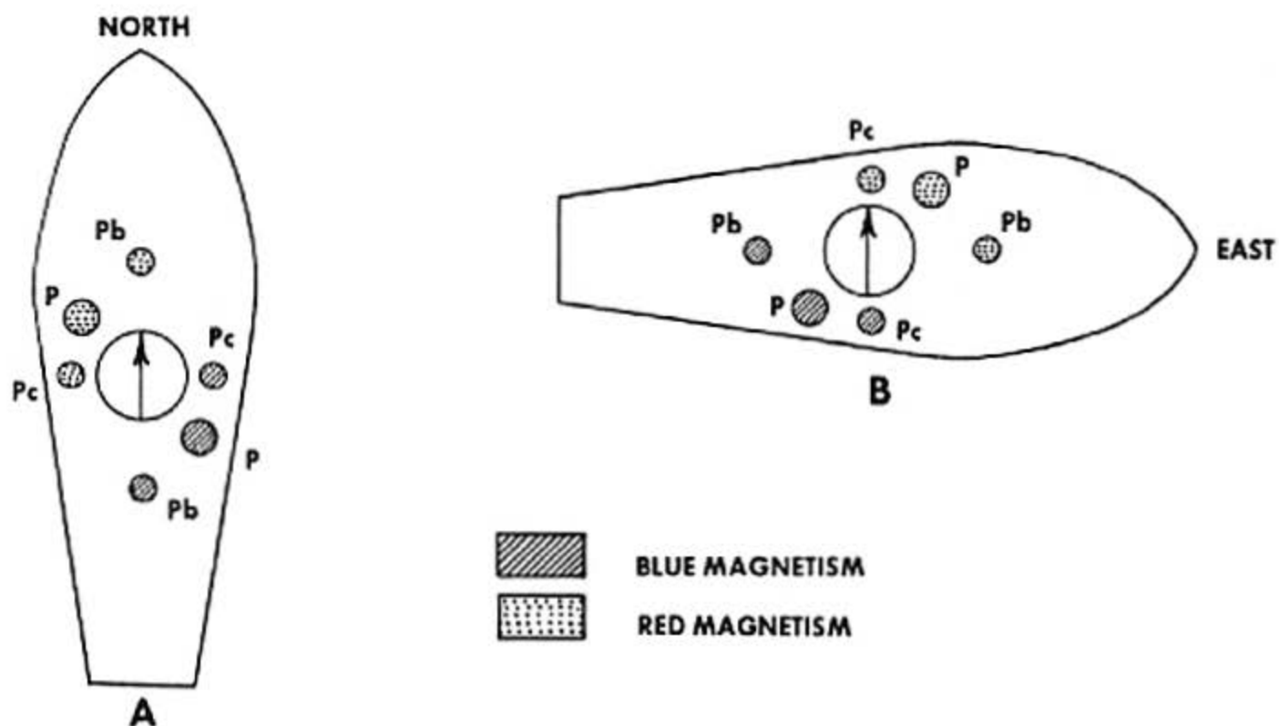
Figure 2-4.—Correcting permanent magnetism.
