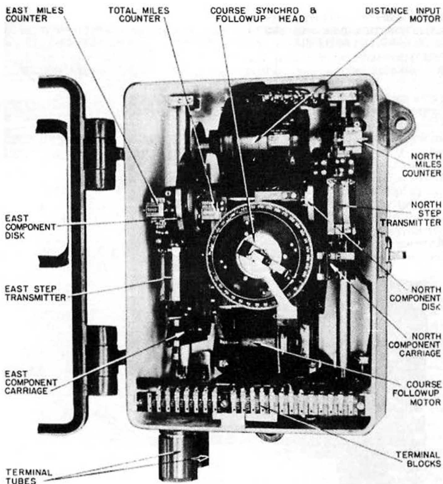
Figure 3-10. DR analyzer. 40.57
