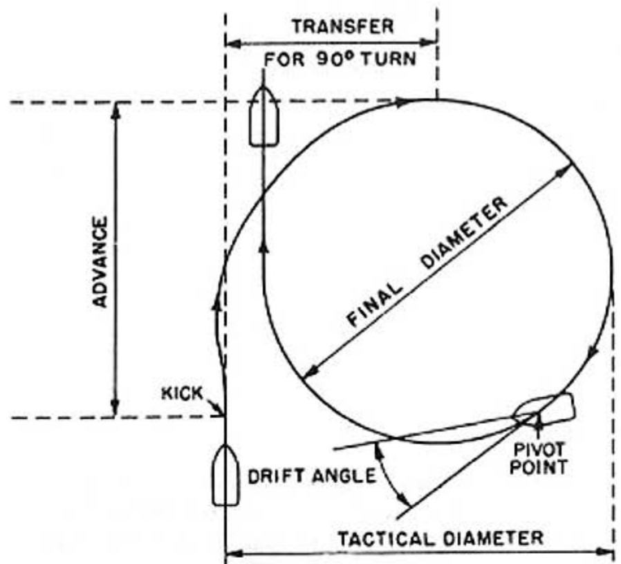
Figure 6-5.—Turning circle. 58.71
