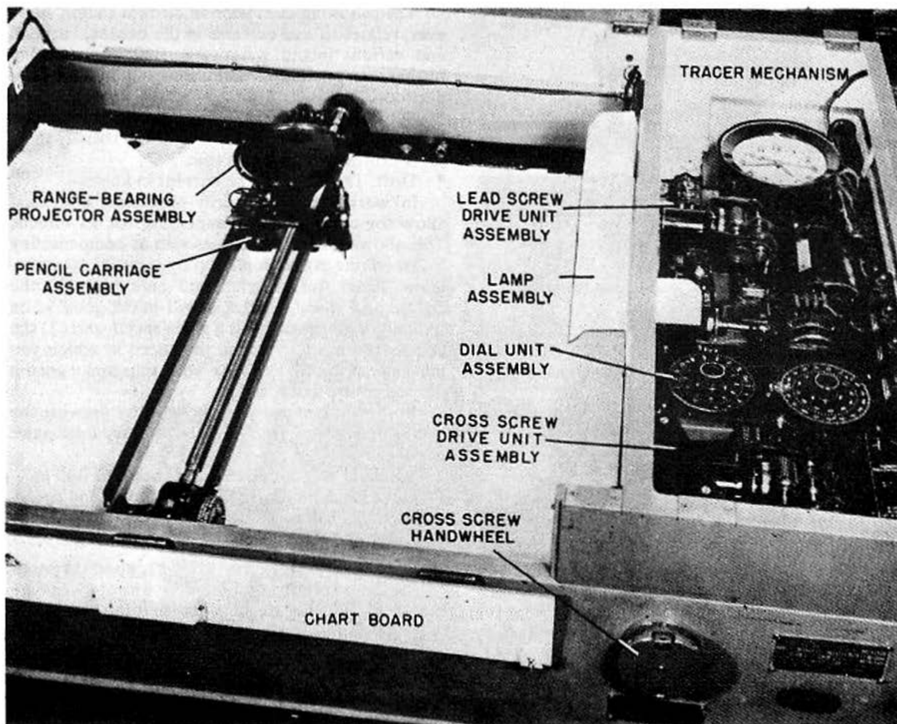
Figure 3-13. DRT plotting table. 40.61
