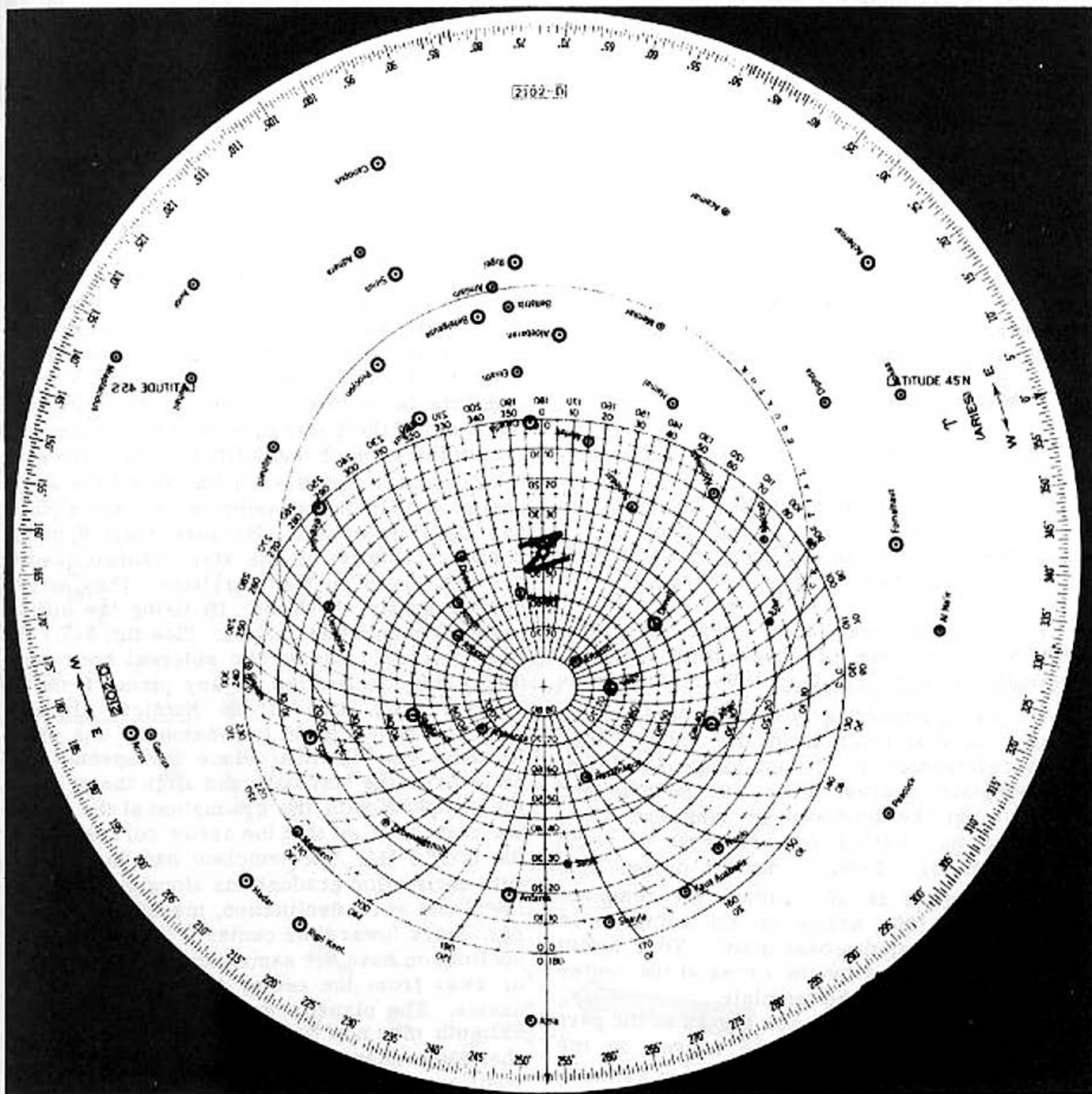
Figure 5-6.—Star finder with template.
