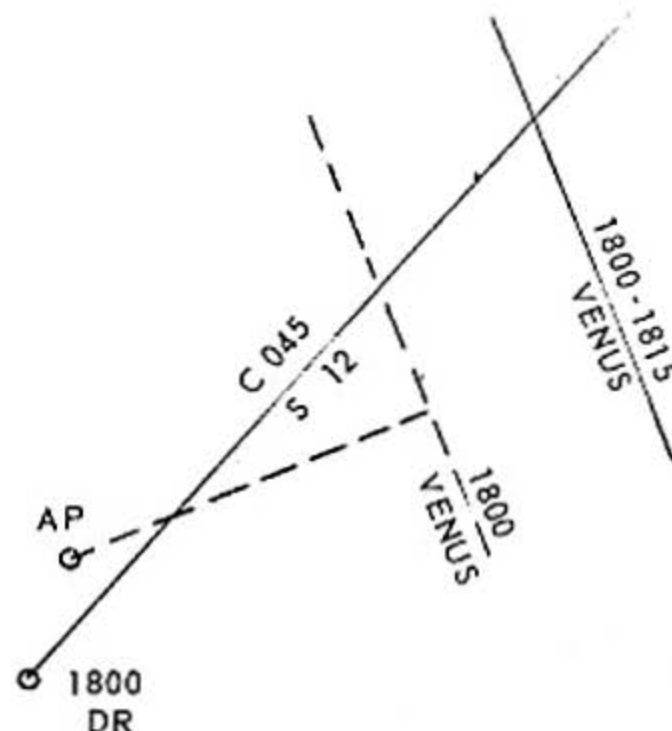
Figure 5-13.—Advancing an LOP. 112.27
