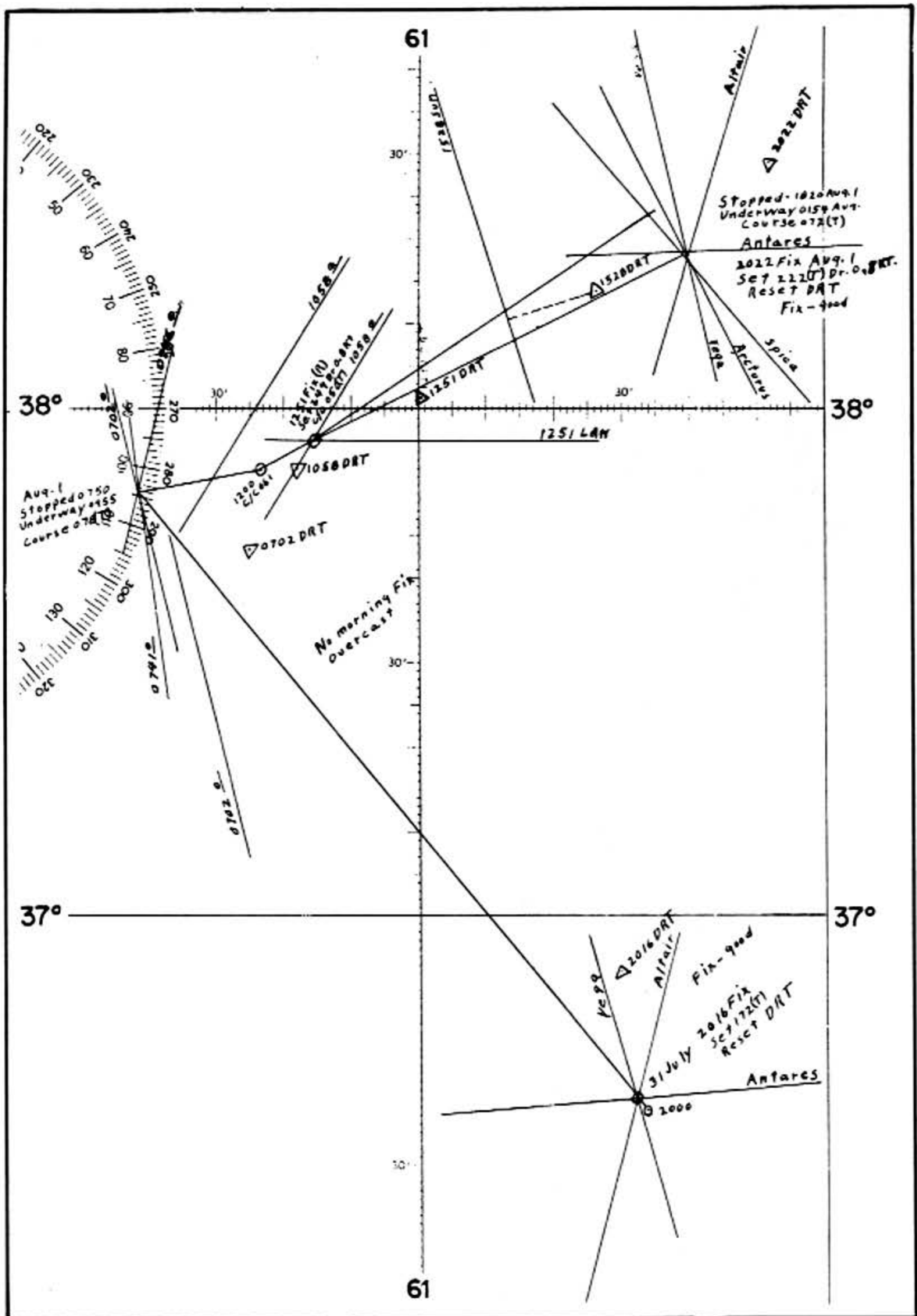
Figure 10-1.—Navigator's worksheet.
