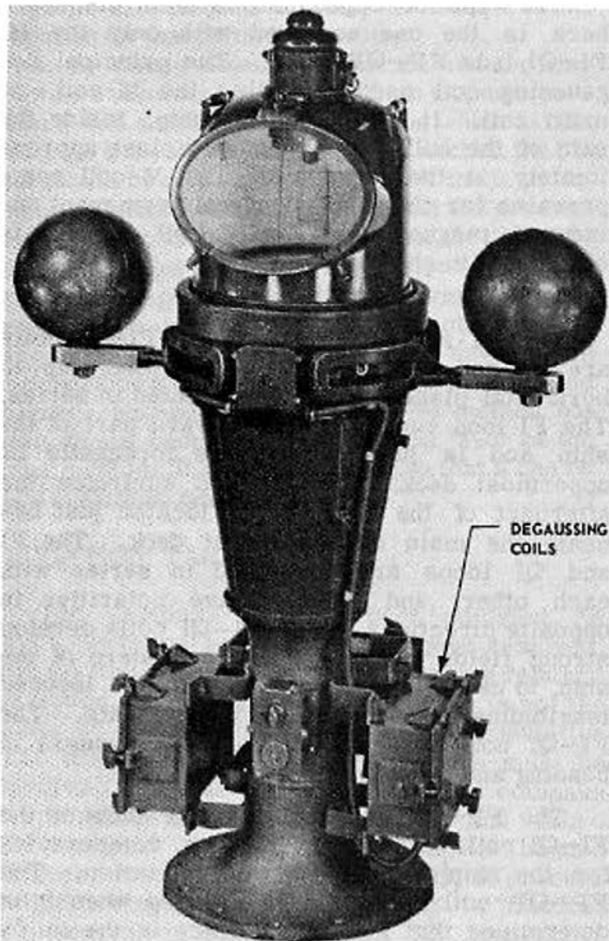
Figure 2-9. Binnacle with degaussing coils. 112.7
