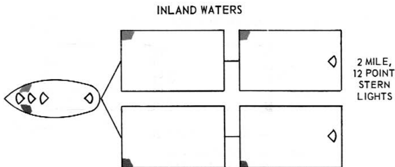
Figure 8-6. Barges abreast in tiers. C80.122
