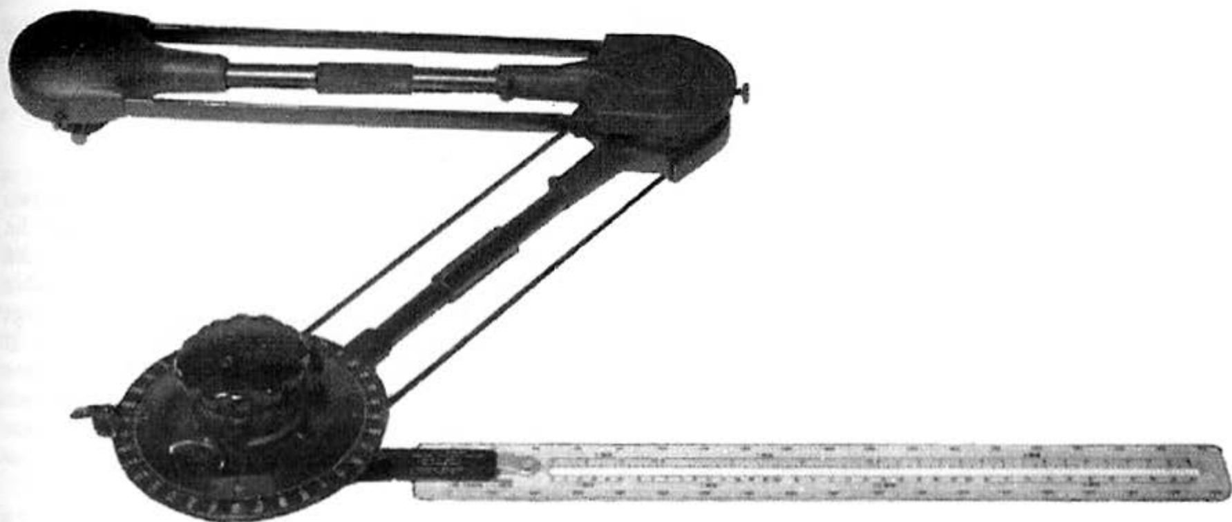
Figure 3-1. Drafting machine. 59.57A
