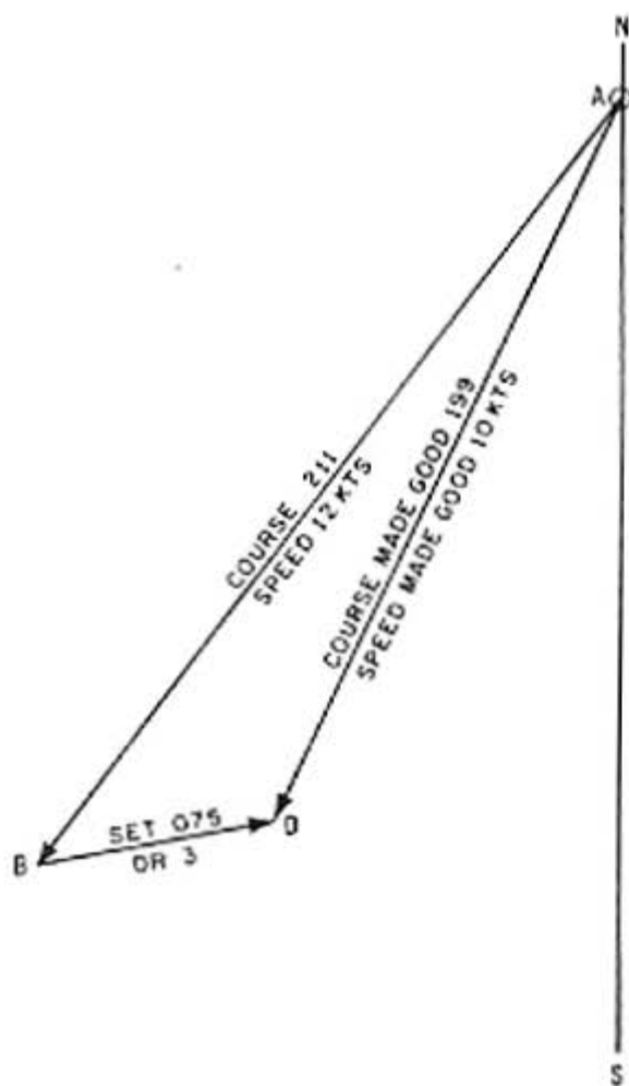
Figure 3-14.—Set and drift problem: Solving for course and speed actually made good.
