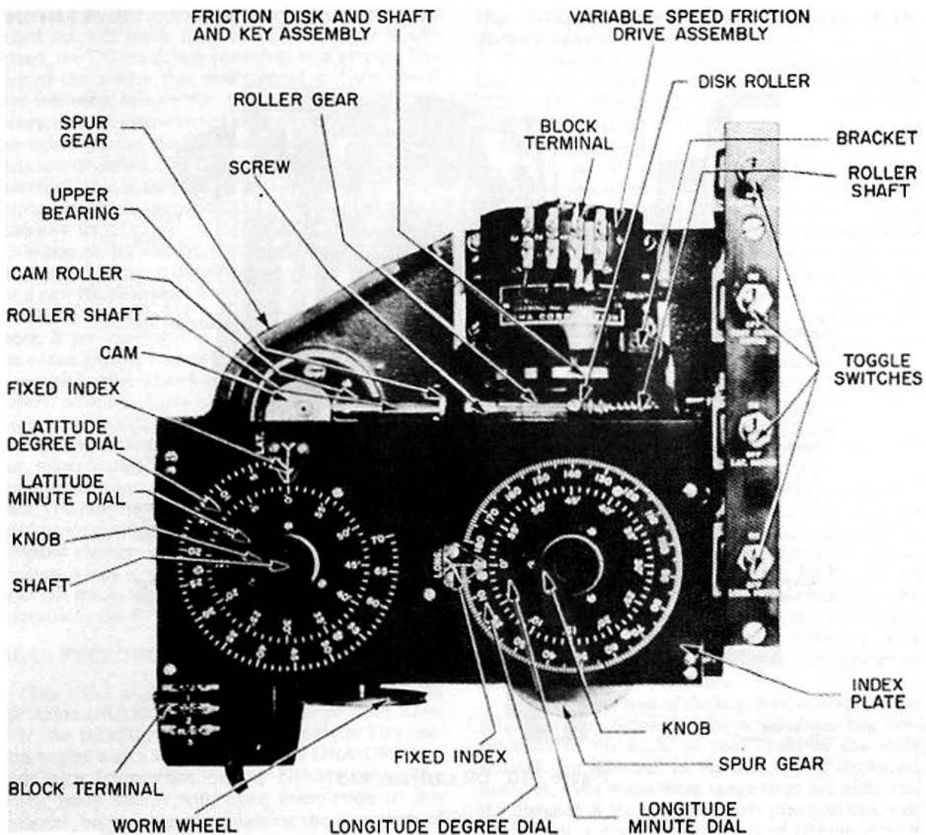
Figure 3-11. DR indicator. 40.59
