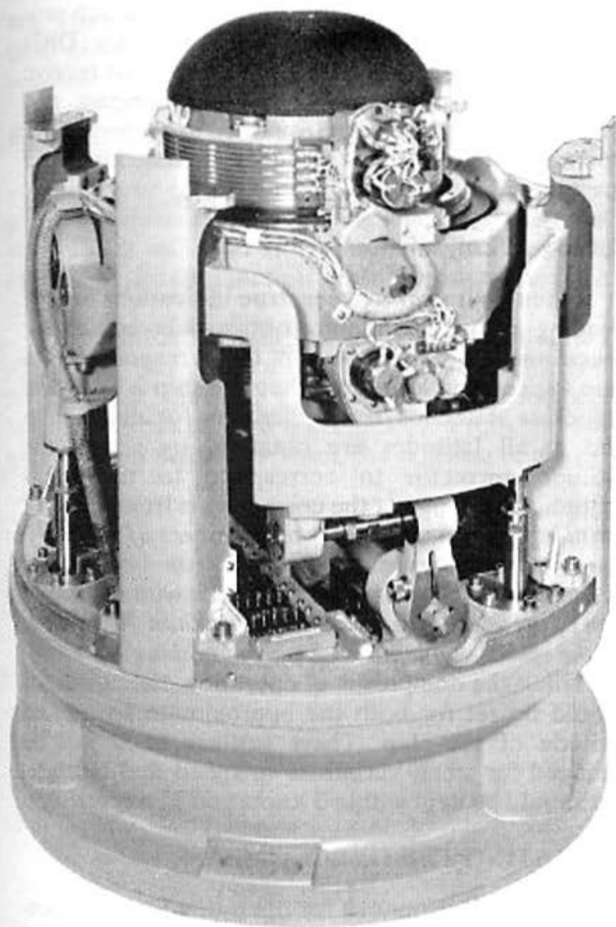
Figure 2-13. Sperry gyrocompass Mk 19.
