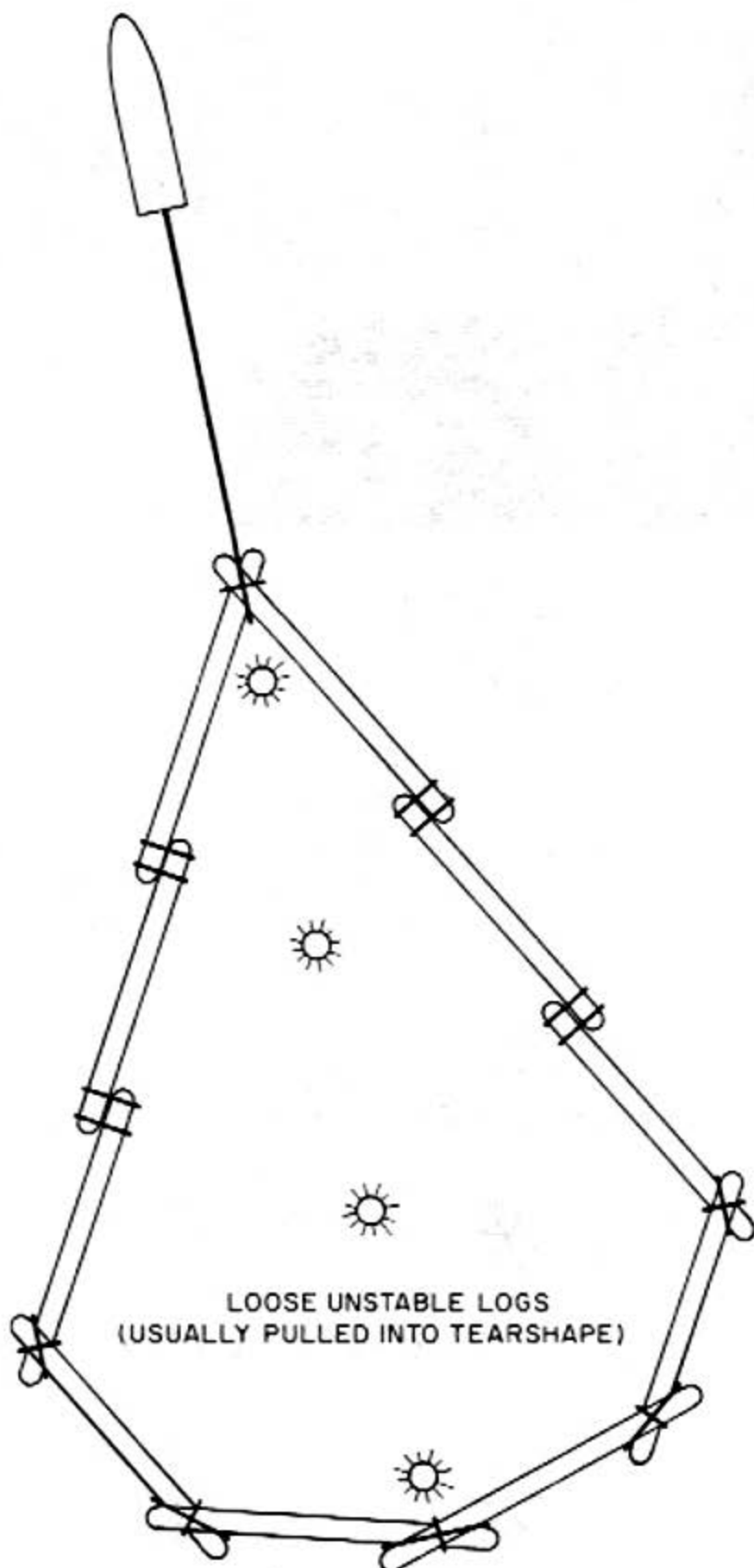
Figure 8-17.—Bag or boom of logs.
