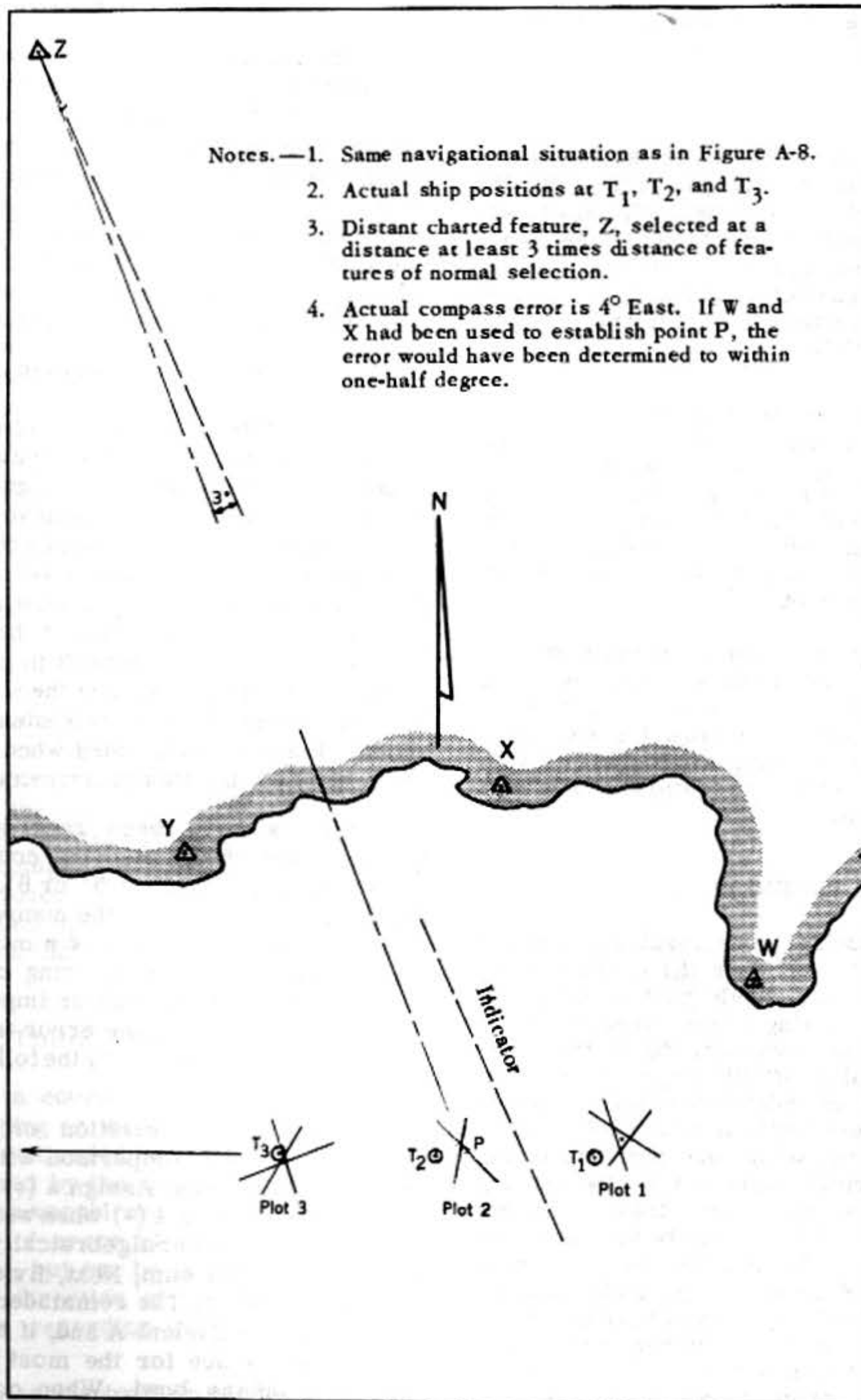
Figure A-9. Direction and approximate magnitude of compass error.
