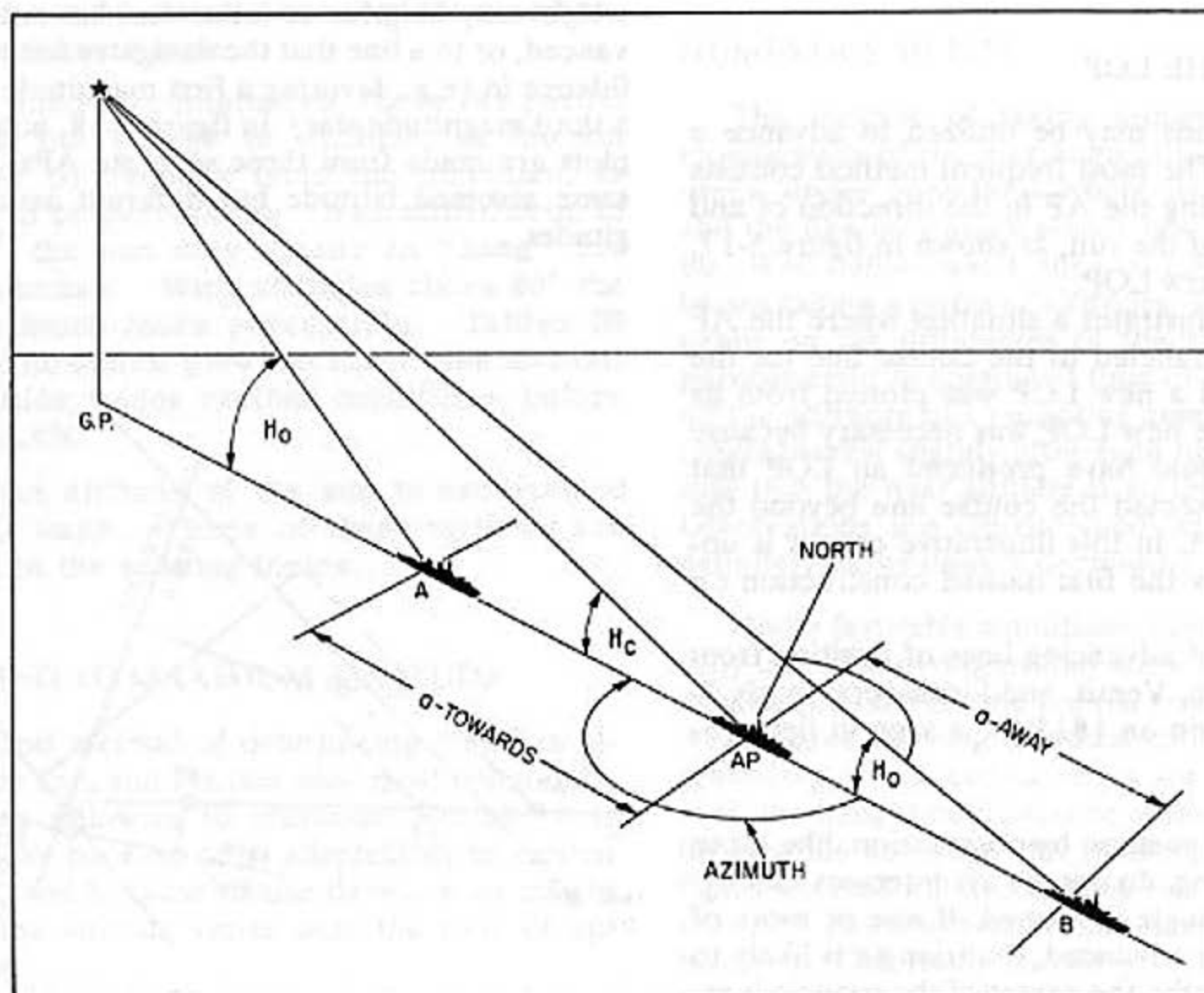
Figure 5-16.—Determining an LOP.
