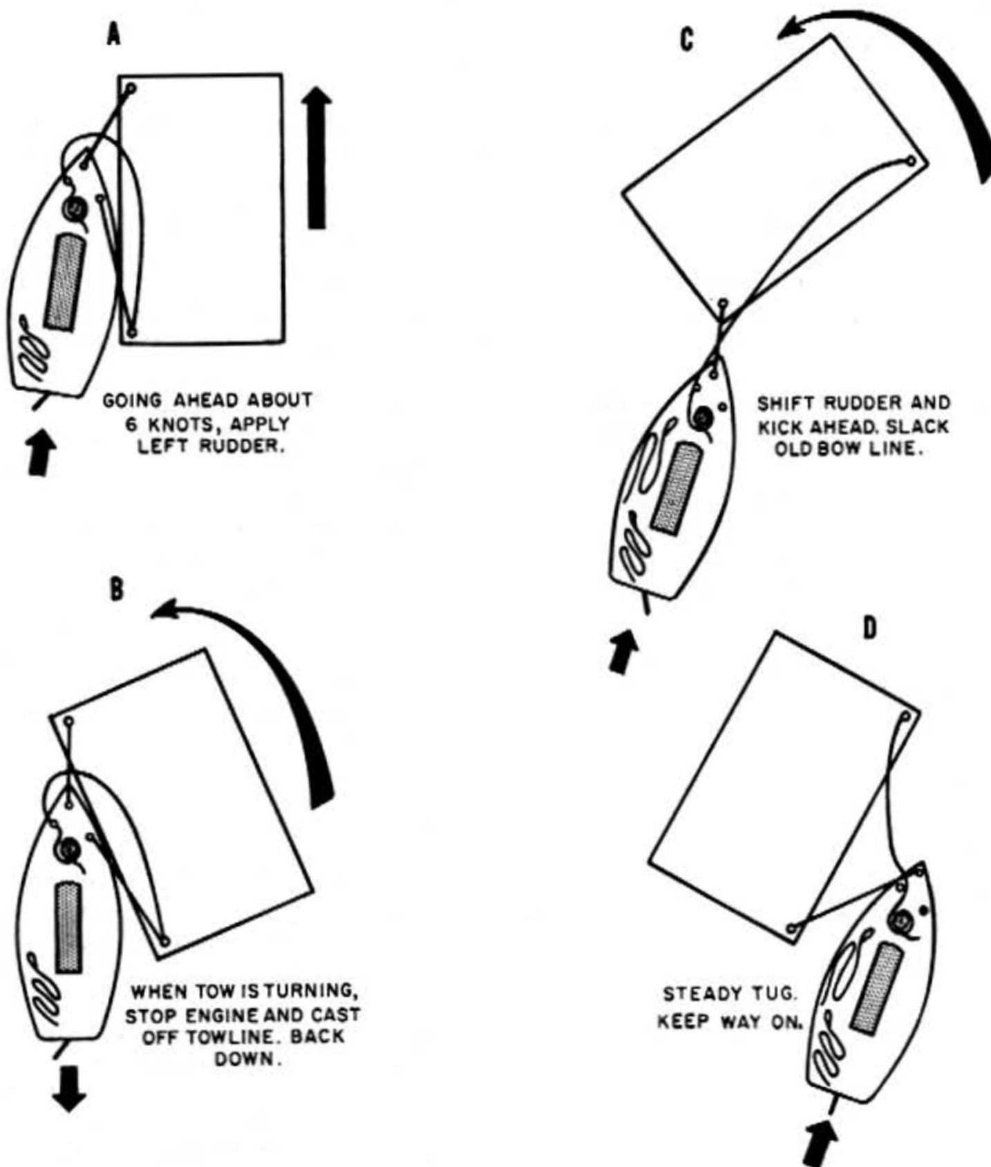
Figure 6-12.—Shifting tow to other side.
