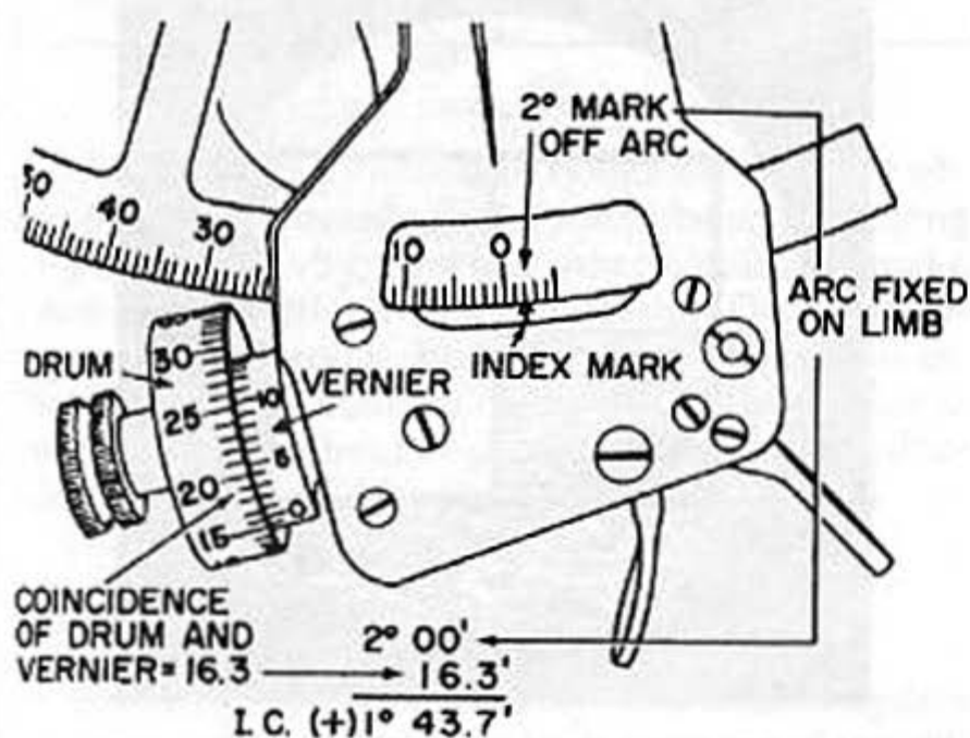
Figure 5-3.—Reading off the arc.
