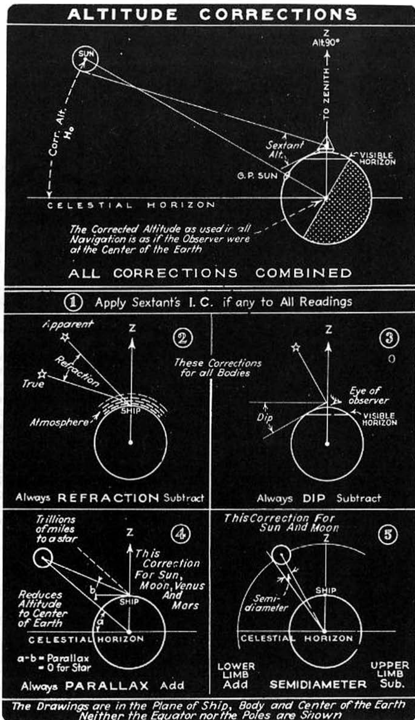
Figure 5-1.—Altitude corrections.
