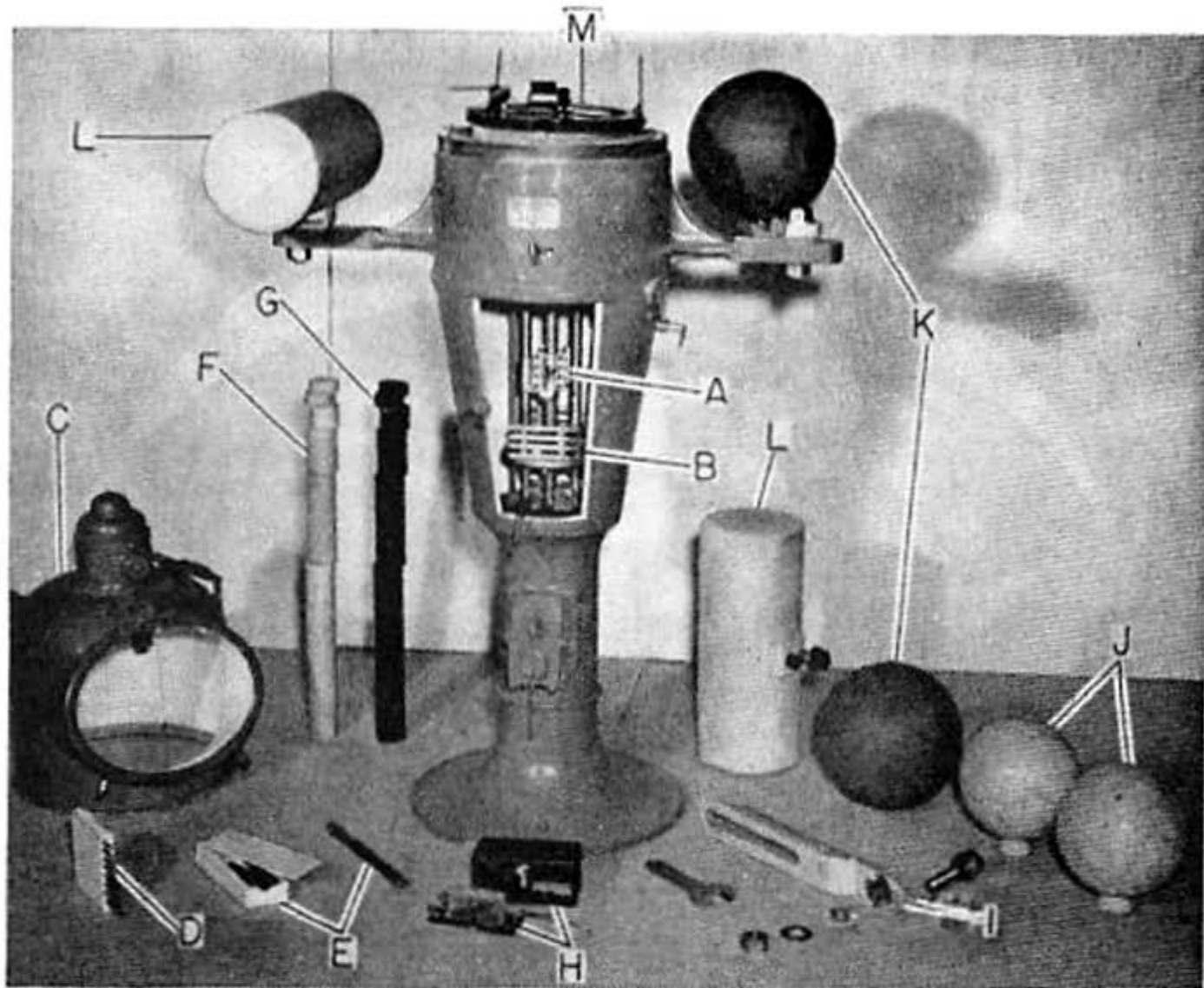
Figure 2-2. Magnetic compass binnacle with correctors. 112.2
