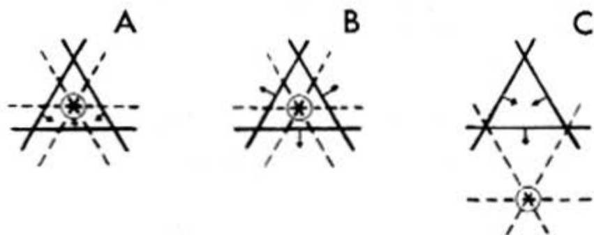
Figure A-5.—Lines of position, shifted to intersect at a common point.
