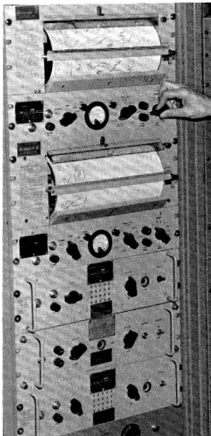
Figure 9-6. FAX receiver employing high-voltage recording stylus. 112.67
