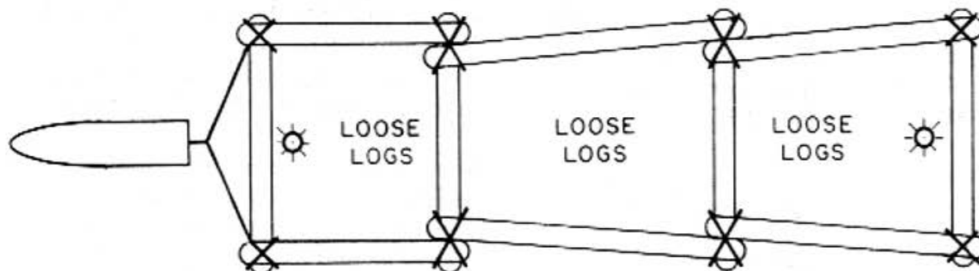
Figure 8-16.—Raft of one crib width.
