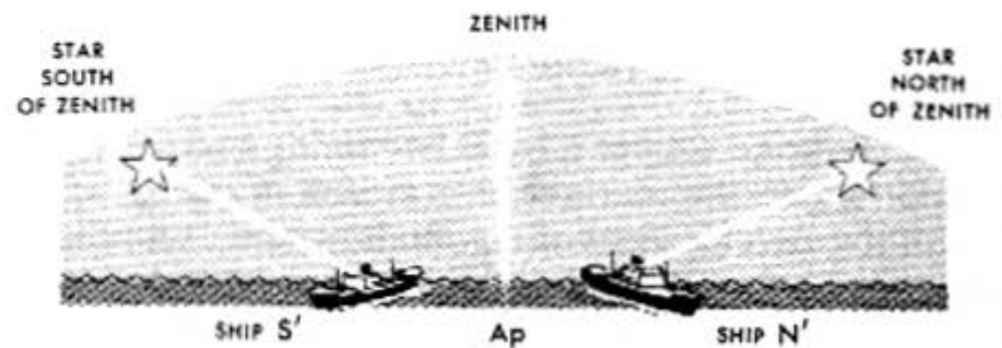
Figure A-2.—Sum of navigator's systematic errors result in observed altitudes that are too high.
