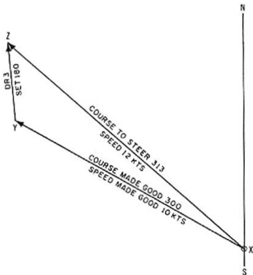
Figure 3-15.—Set and drift problem: Solving for course to steer and steaming speed.
