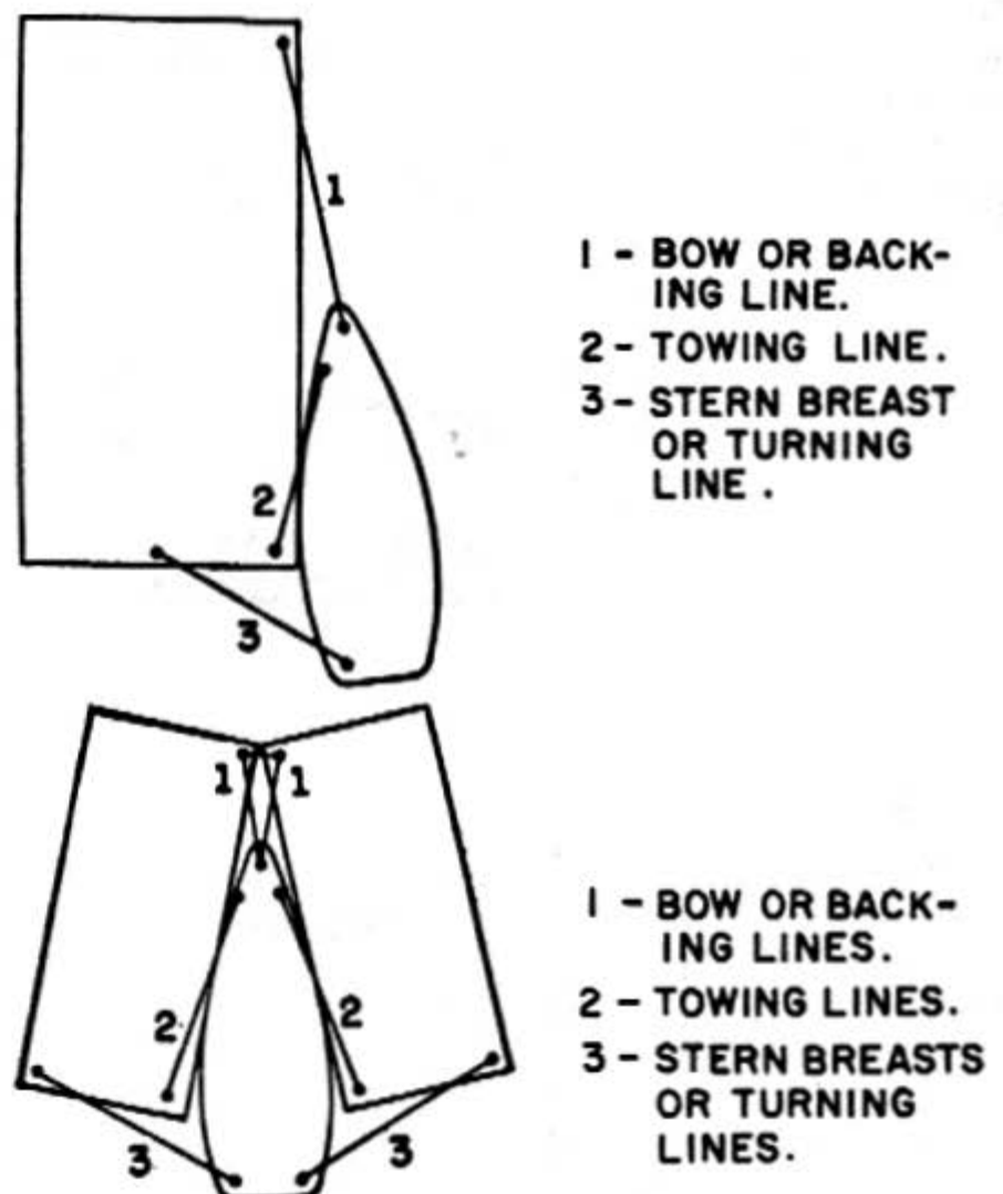
3.227(58)D Figure 6-11.—Alongside towing.
