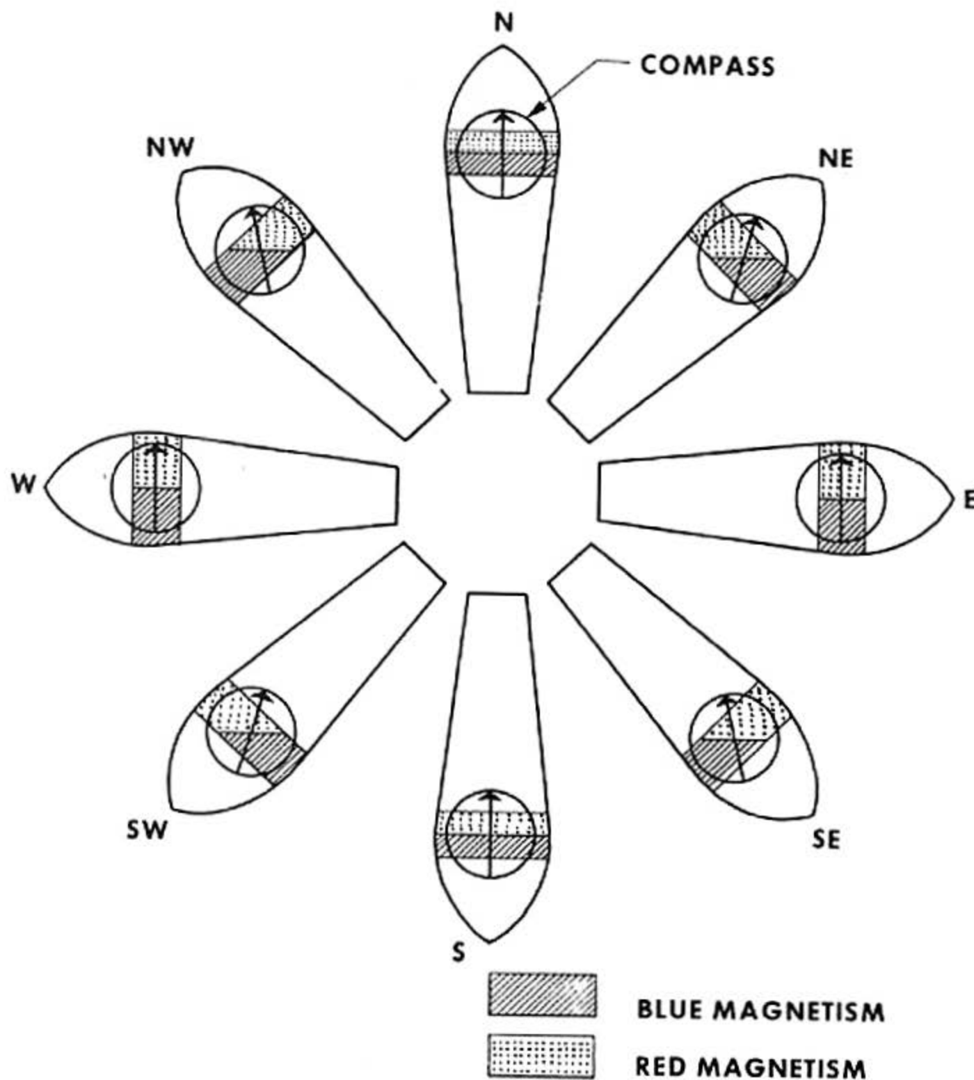
Figure 2-5.—Quadrantal deviation.
