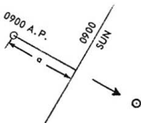
Figure 5-10.—Plotting a sun LOP. 112.24
