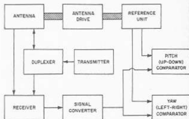
Figure 9-15.—Active homing system; block diagram.
