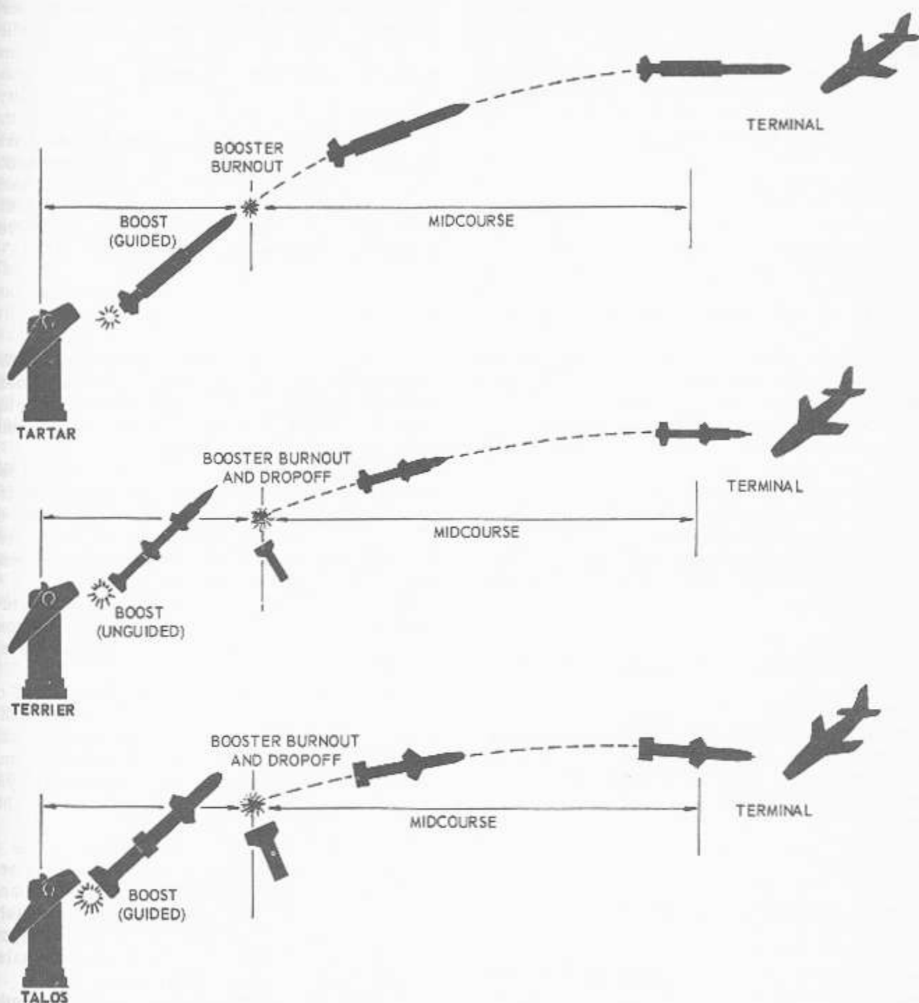
Figure 6-1.—Guidance phases of missile flight.
