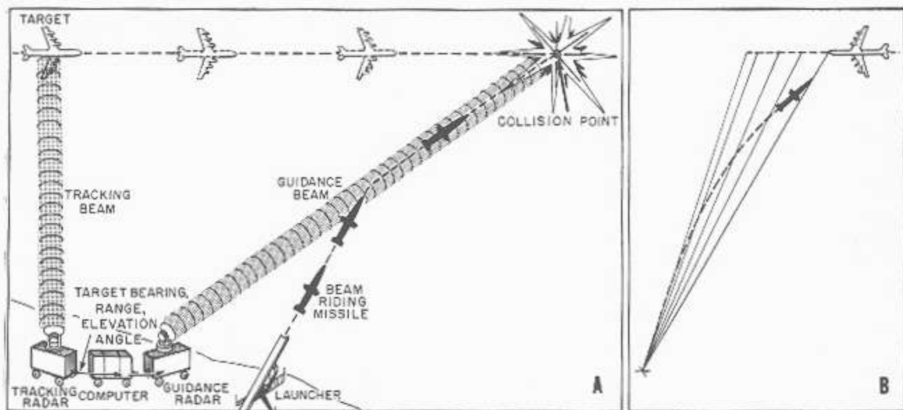
Figure 8-21.—Beam-rider guidance: A. Two-radar beam riding guidance; B. The programmed beam-rider.
