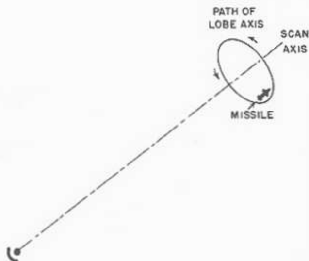
Figure 8-10.—Missile below the scan axis.
