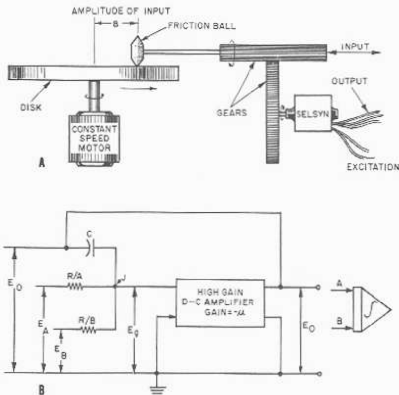
Figure 5-28.—Some integrators used in missile control: A. Ball-and-disc integrator; B. Integrating amplifier circuit and symbol.
