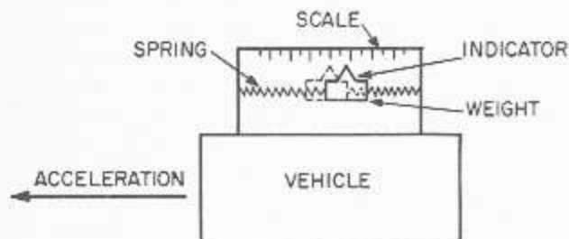
Figure 10-4.—Elementary accelerometer, spring-mounted.
