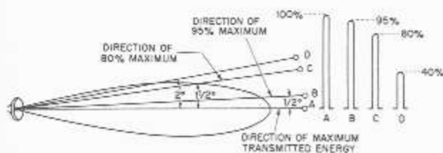
Figure 8-16.—Variation in radiated energy with distance from lobe axis.
