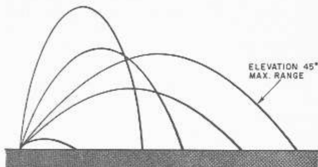
Figure 10-2.—Theoretical trajectories at various gun elevations (ignoring air resistance).
