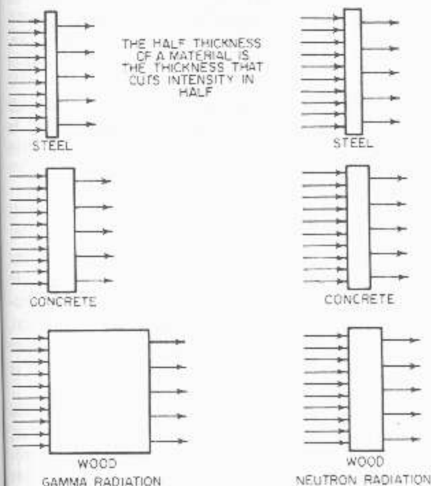
Figure 12-10.—Typical examples of relative half thickness.
