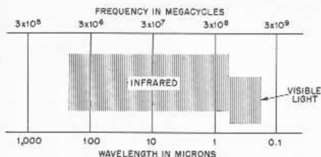
Figure 9-3.—Infrared portion of electromagnetic spectrum.
