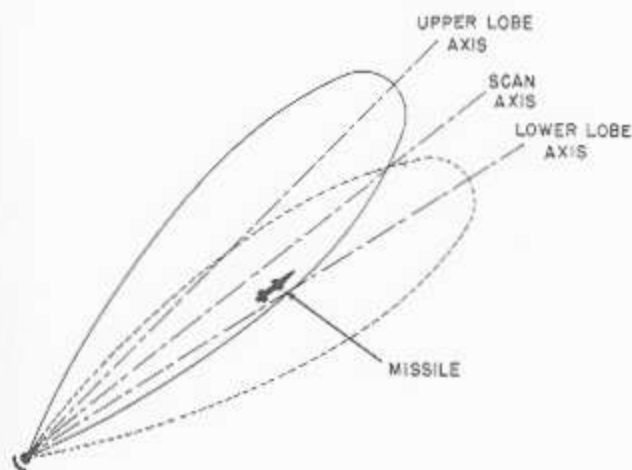
Figure 8-11.—Two-lobe scanning system.
