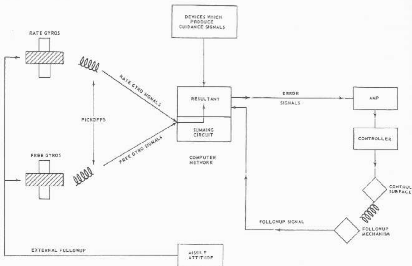
Figure 5-27.—Missile control system showing gyros and pickoffs.
