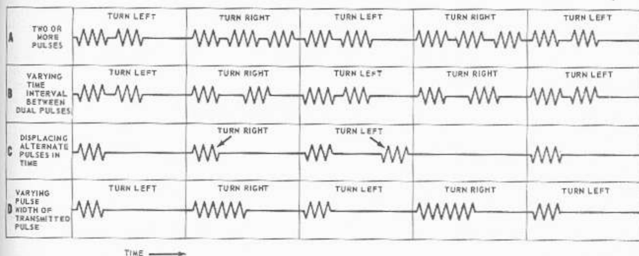
Figure 7-6.—Methods of transmitting commands by radar pulses.
