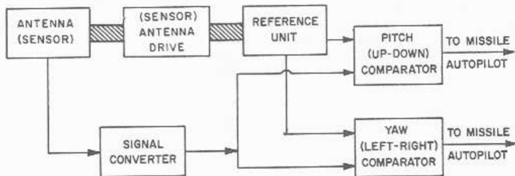
Figure 9-10.—Passive homing guidance system, block diagram.
