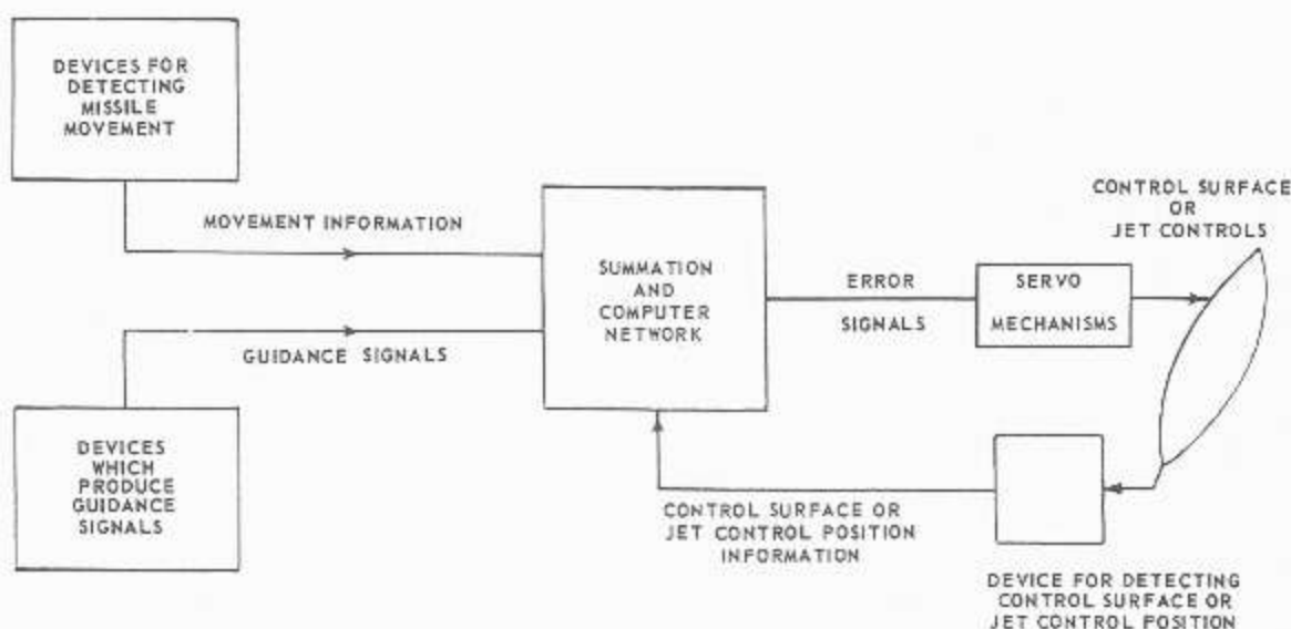
Figure 5-1.—Simplified missile control system.
