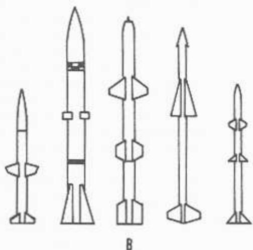
Figure 2-10.—Control surfaces: A. Fixed and movable surfaces; B. Control surface designs and locations.
