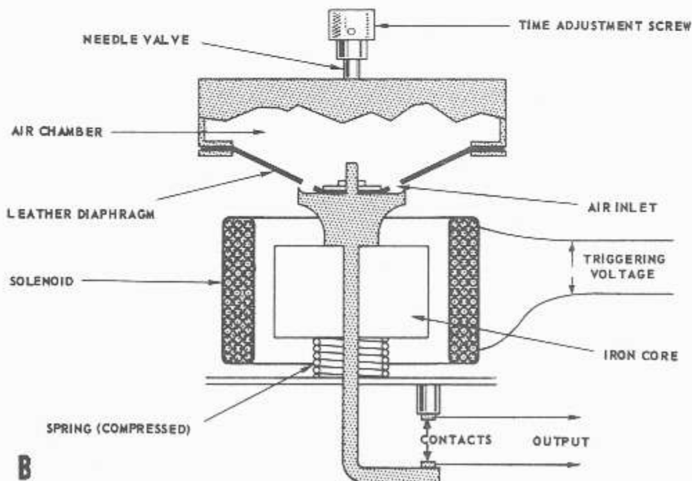
Figure 5-13.—Pneumatic timers: A. Piston type pneumatic timer; B. Diaphragm timer.
