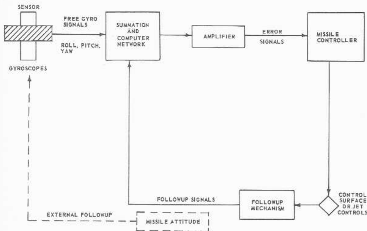
Figure 5-9.—Basic missile control system.
