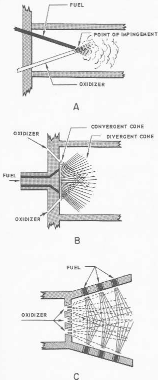
Figure 4-6.—Types of injectors in liquid-fuel rockets: A. Multiple hole impingement injector; B. Spray injector; C. Non-impinging injector.
