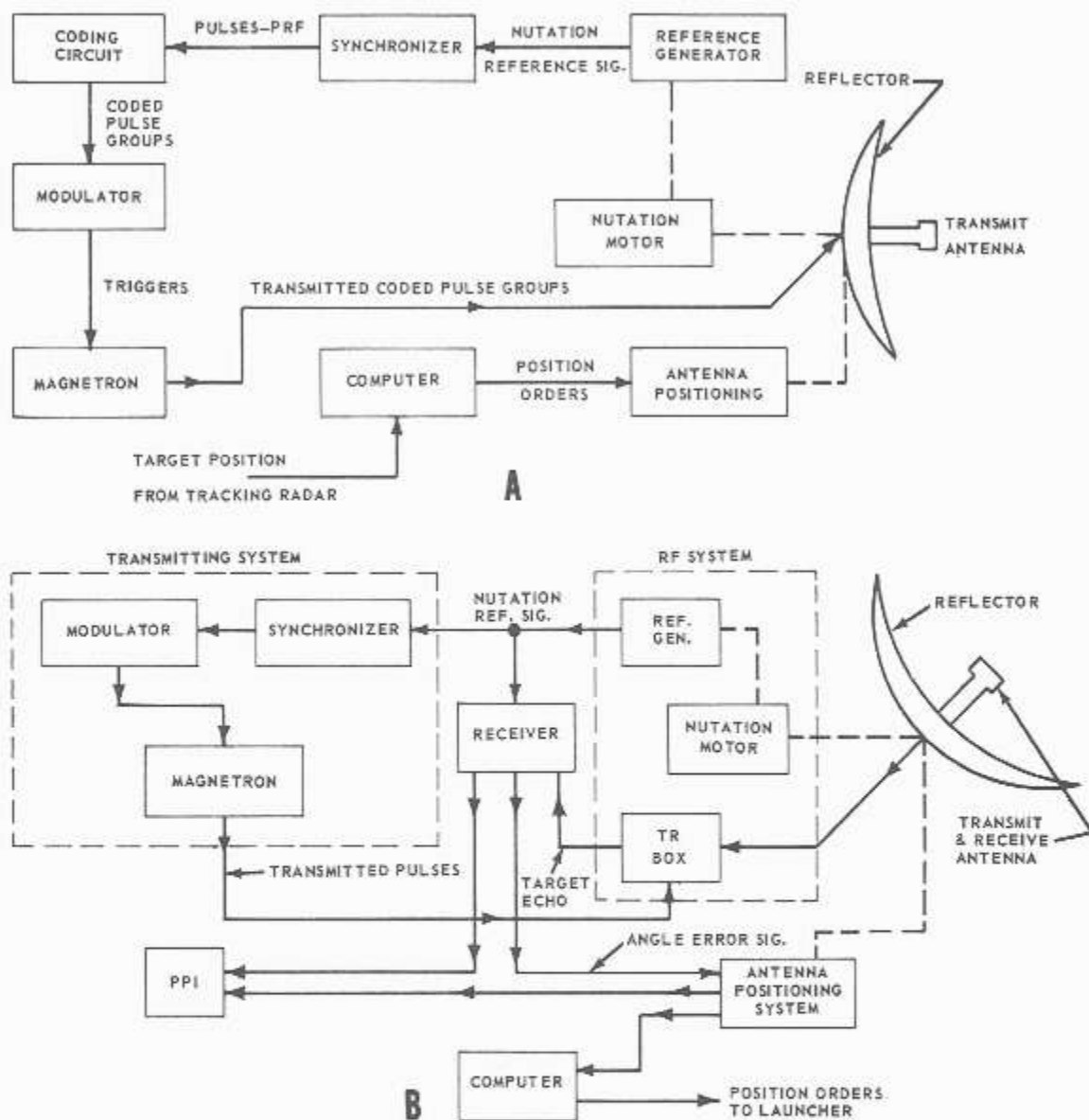
Figure 8-15.—Block diagrams of weapon system radars: A. Control radar; B. Tracking radar. 33,150
