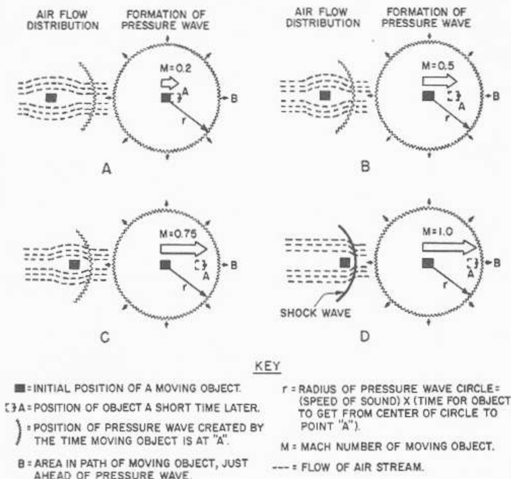
Figure 2-12.—Compressibility of air at various speeds.
