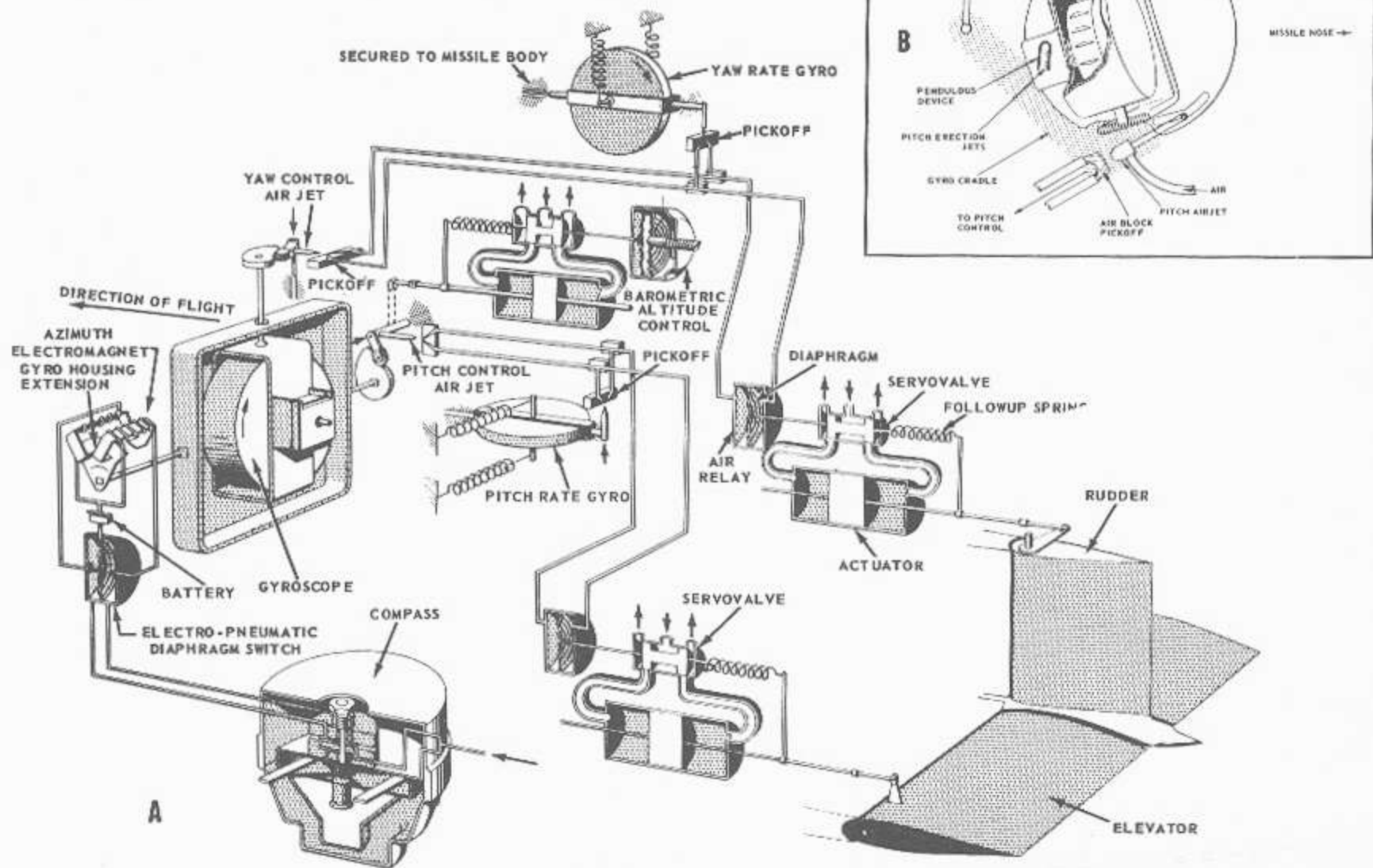
Figure 5-40.—A. Pneumatic control system; B. Detail of pitch control assembly.
