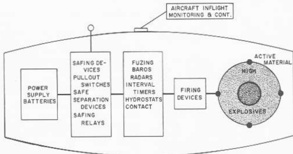
Figure 13-2.—Idealized implosion type weapon.
