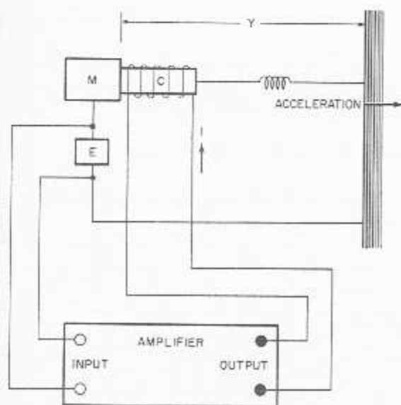
Figure 6-11.—Electrically damped accelerometer.
