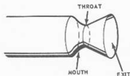
Figure 4-3.—Location of nozzle areas.
