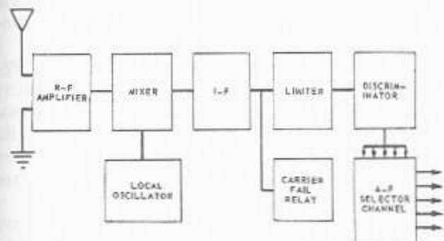
Figure 7-3.—Command receiver in missile.
