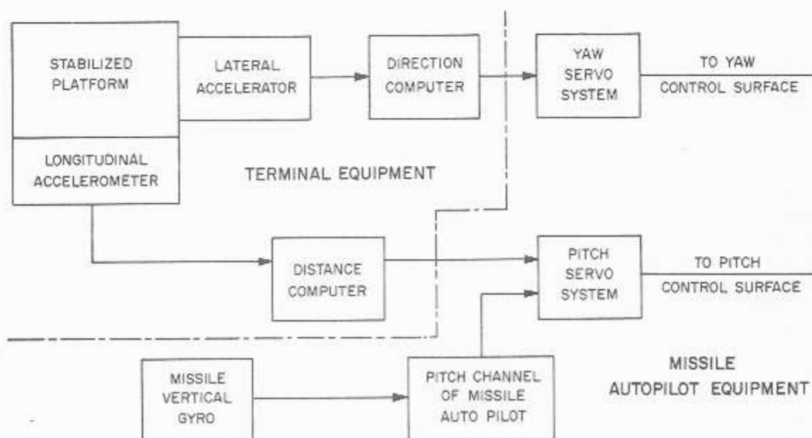
Figure 10-12.—Constant-dive-angle system for missiles.
