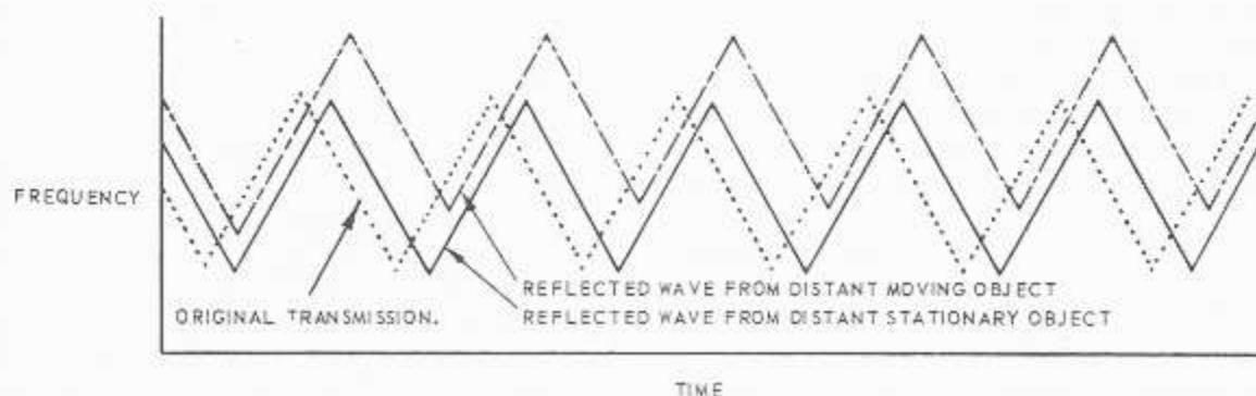
Figure 6-16.—Doppler effect on frequency modulation (sawtooth wave).
