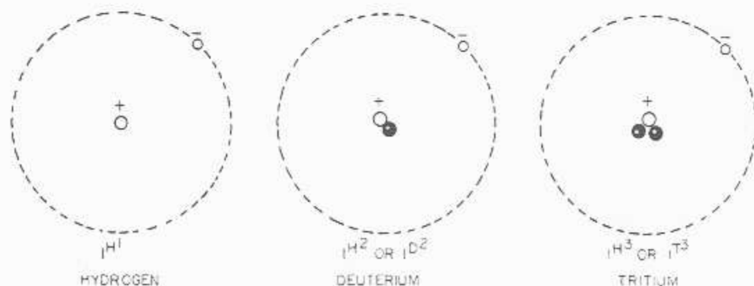
Figure 12-5.—The three hydrogen isotopes.
