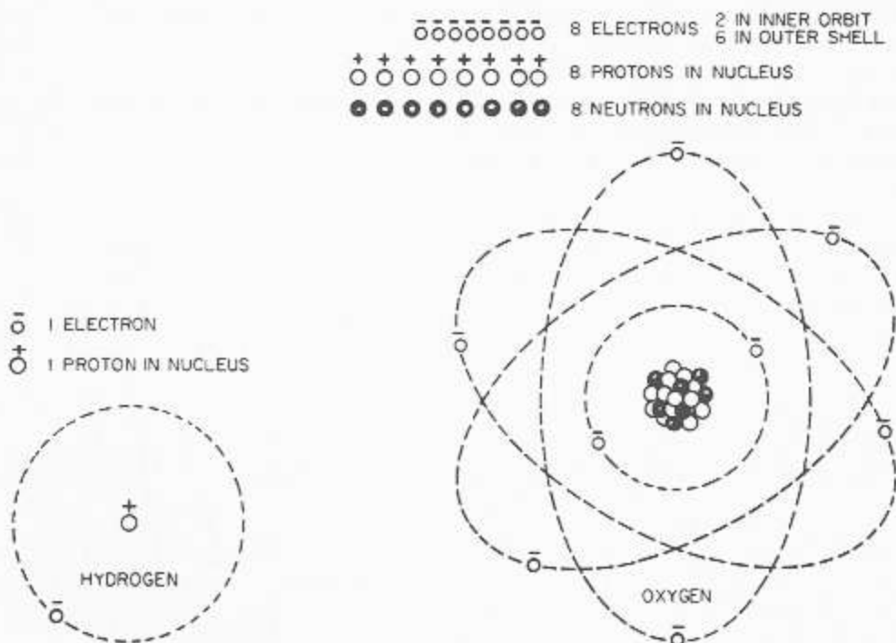
Figure 12-2.—Electron relationship of atoms.
