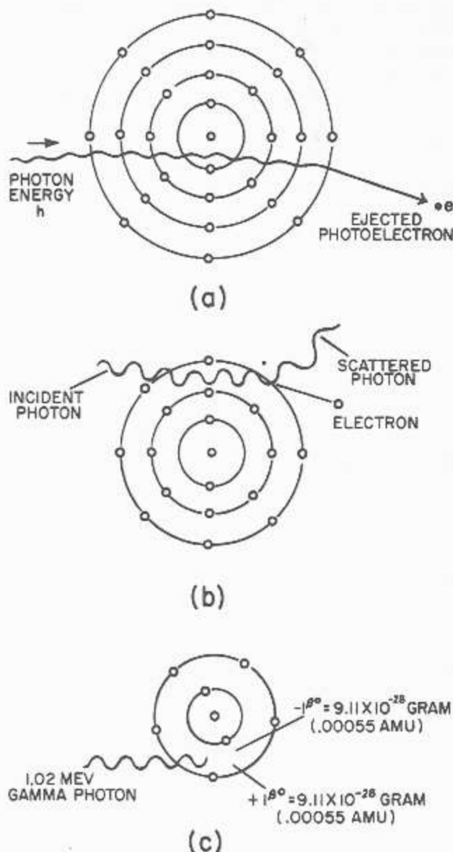
5.159:160 Figure 12-6B.—Absorption of gamma rays, showing (a) photoelectric effect; (b) Compton effect; (c) pair production.
