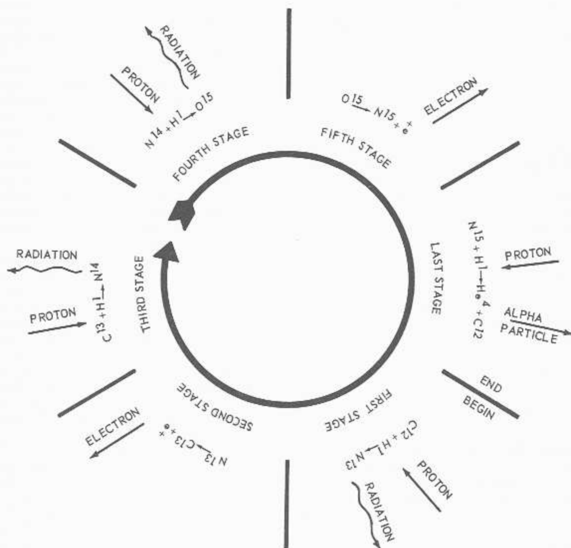
Figure 13-3.—Fusion in the sun.
