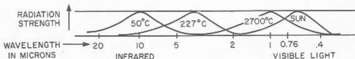
Figure 9-4.—Infrared radiation at different temperatures.
