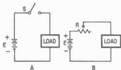
Figure 5-7.—Elementary control circuit: A. Discontinuous control; B. Continuous control.
