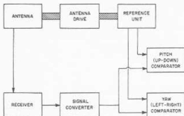
Figure 9-14.—Semicative homing systems; block diagram.
