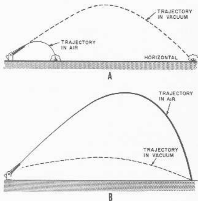
Figure 10-3.—Comparison of vacuum and air trajectories: A. In range; B. In elevation.
