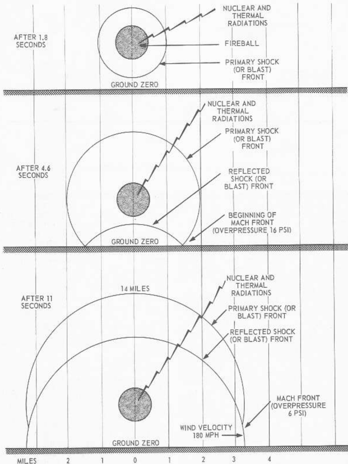
Figure 14-2.—Three stages in the development of a 1-megaton air burst at 6,500 feet height.
