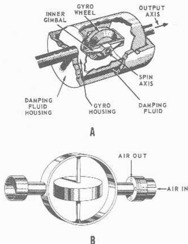
Figure 5-17.—Friction-reducing gyro units: A. Floated gyro unit; B. Air breathing gyro.
