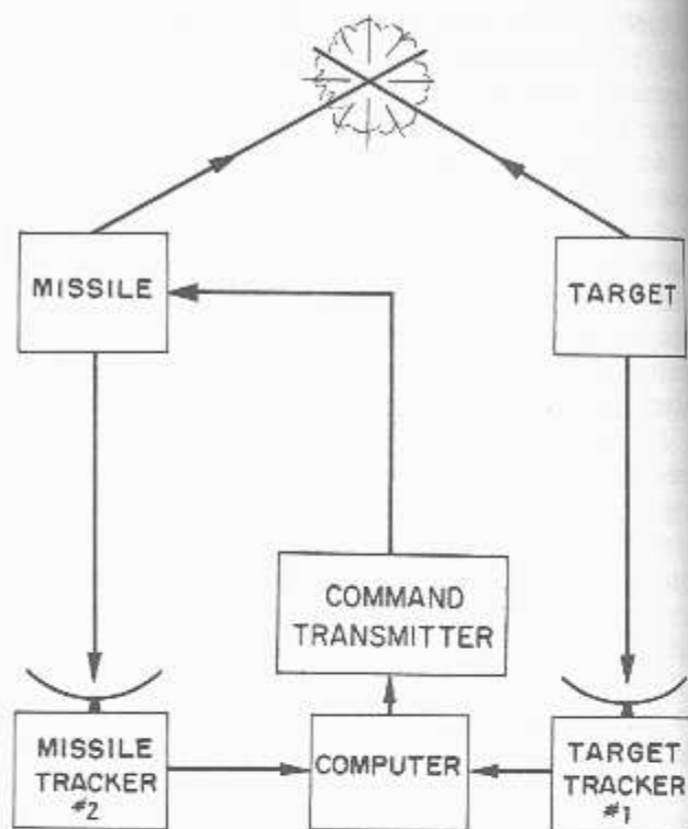
Figure 6-5.—Command guidance system.
