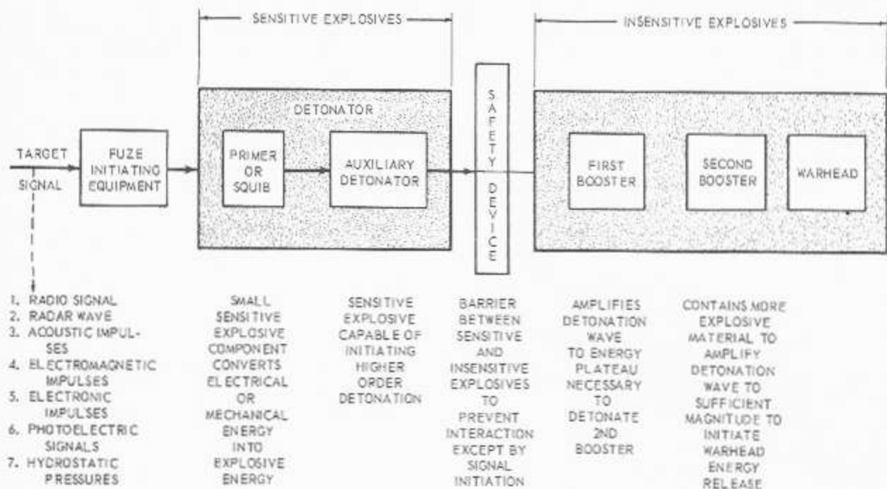
Figure 3-10.—Schematic of typical explosive train with safety device.
