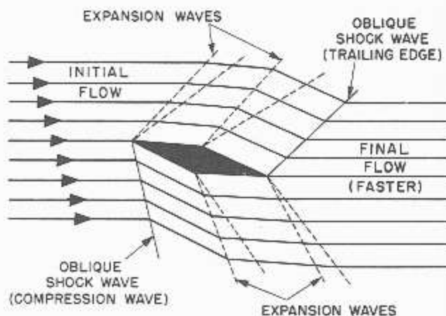
Figure 2-16.—Airflow about a supersonic fin.
