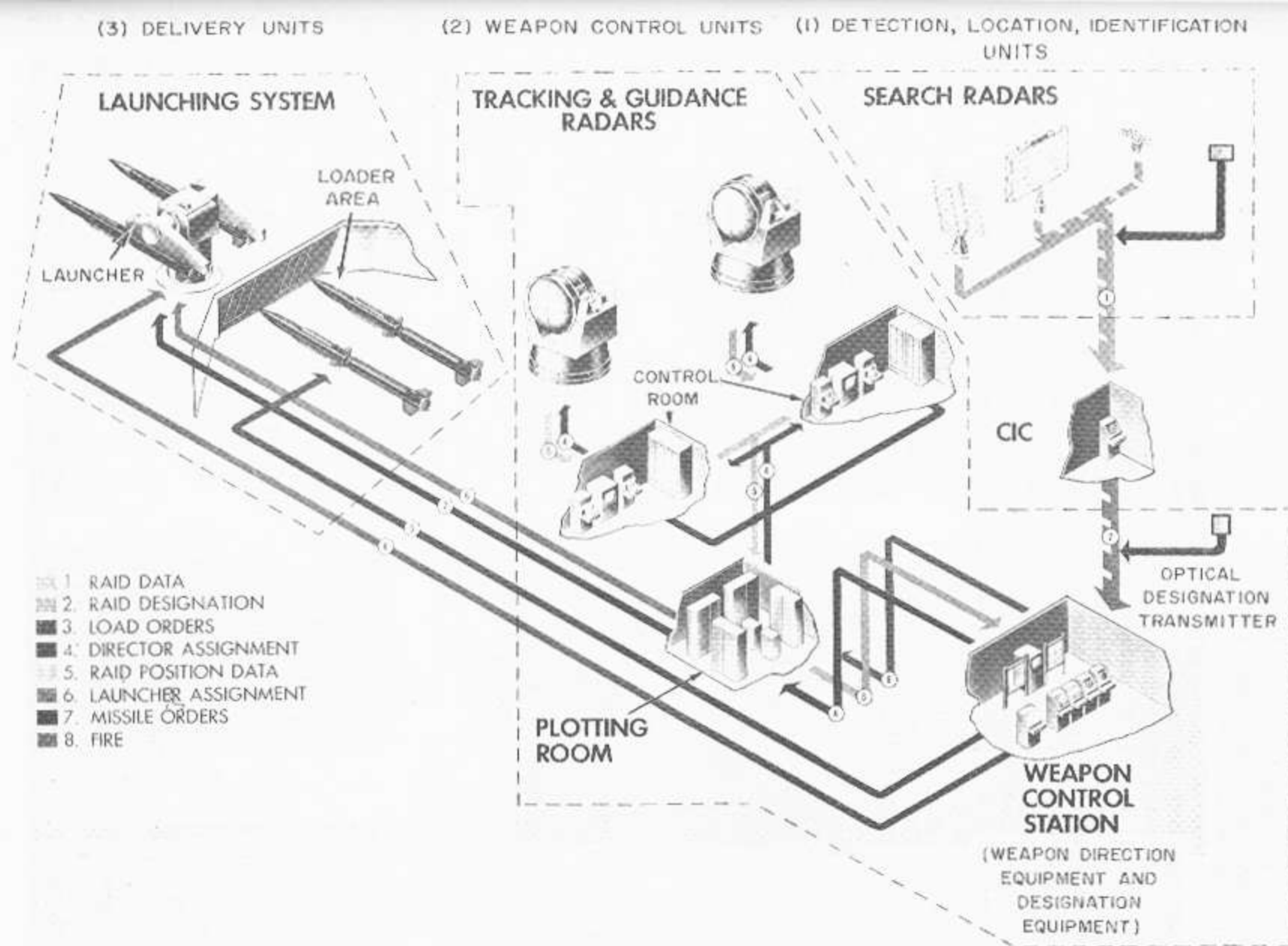
Figure 11-12.—Terrier weapons system, flow of information and directions.
