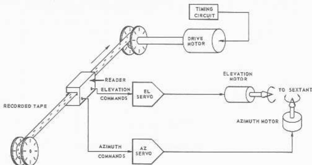
Figure 10-17.—Sextant-positioning system.
