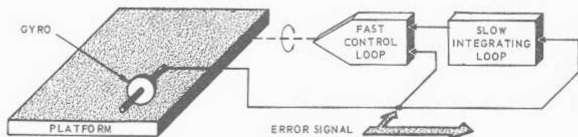
Figure 10-9.—Gyro-drift compensation. 144.51
