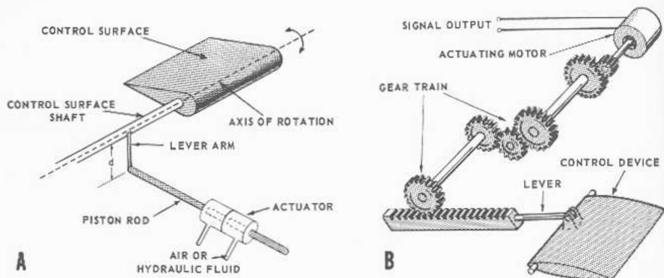
Figure 3-43.—Mechanical linkages: A. Actuator and load linked by lever arm; B. Gear train type of mechanical linkage.
