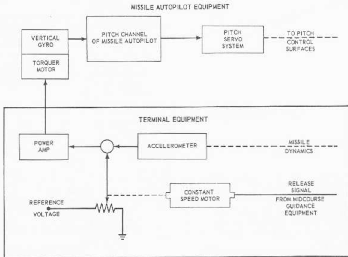
Figure 10-14.—Zero-lift inertial system.
