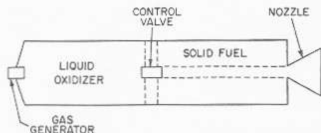
Figure 4-16.—Sketch of a hybrid propulsion engine.
