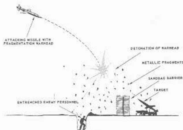
Figure 3-4.—Effect of fragmentation warhead on surface target.
