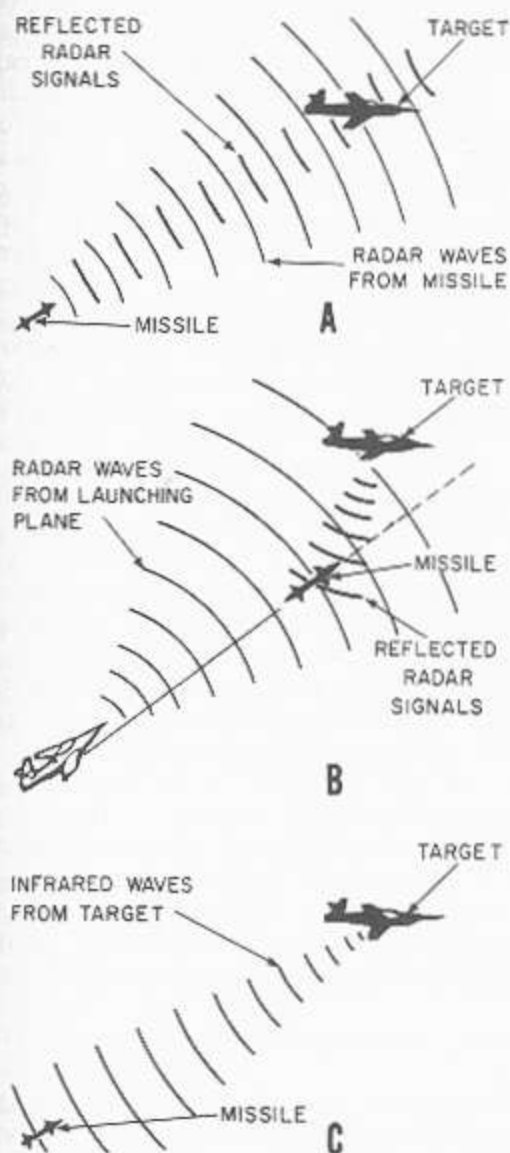
Figure 6-8.—Homing guidance: A. Active homing; B. Semiactive homing; C. Passive homing.
