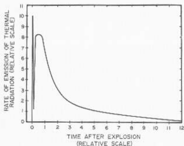
Figure 14-15.—Emission of thermal radiation in two pulses in an air burst.
