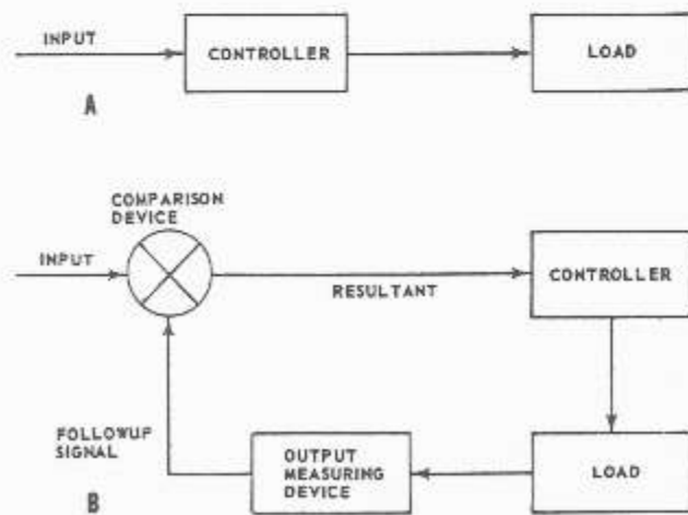
Figure 5-8.—Basic types of automatic servo-systems: A. Open-loop; B. Closed-loop.
