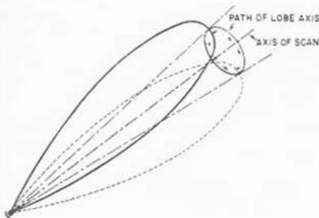
Figure 8-6.—Nutating lobe, conical scanning.
