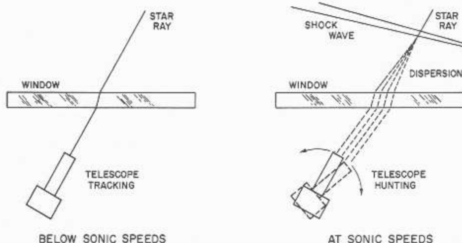
Figure 10-19.—Effect of high speeds on optical systems.
