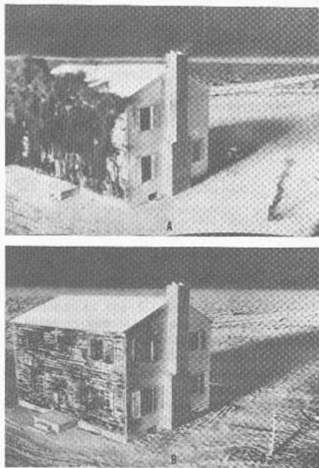
Figure 14-18.—Effects of thermal radiation on white-painted exterior of wood frame house: A. Almost immediately after explosion; B. Effects as seen about 2 seconds later.
