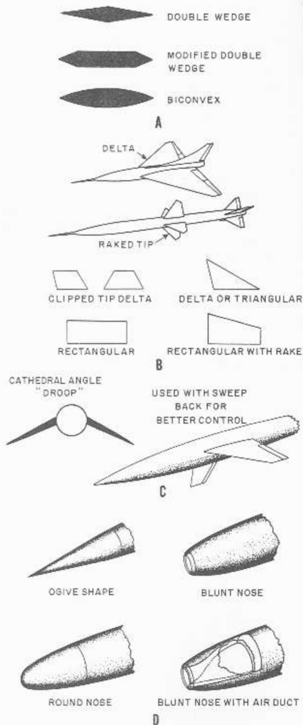
33.33-.41 Figure 2-22.—High speed configuration characteristics: A. Supersonic fin cross-sectional shapes; B. Supersonic fin platforms; C. Wing angle; D. Missile noses.
