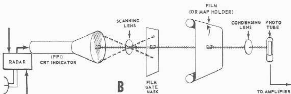
Figure 10-20.—Radar mapmatching: A. Block diagram of system; B. Film holder operation for strip map.
