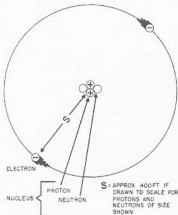
Figure 12-4.—Typical simple atom. 144.60
