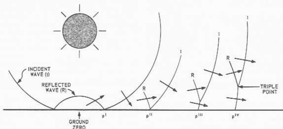
Figure 14-3.—Formation of the Mach front.
