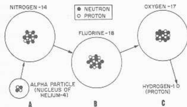
Figure 12-7.—Artificial or induced radioactivity. A. Bombardment of a nitrogen 14 atom with an alpha particle; B. The alpha particle is momentarily absorbed, forming fluorine 18; C. One proton cast off, leaving oxygen 17.
