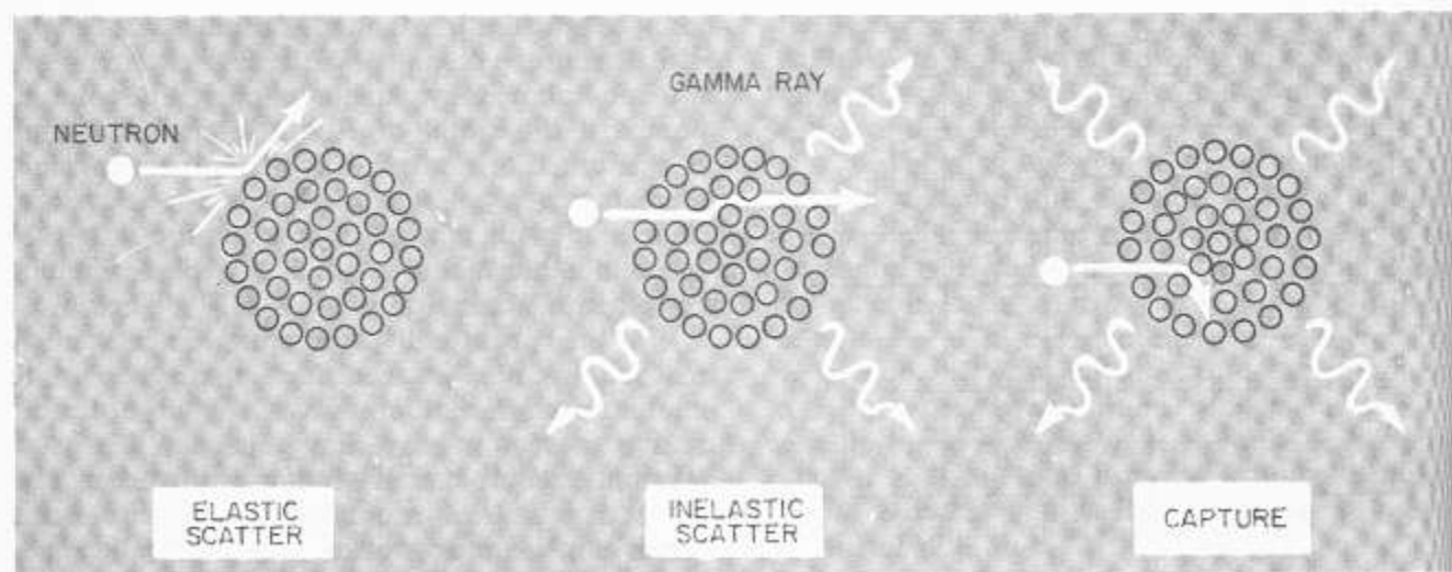
Figure 12-13.—Some non-fissioning reactions.
