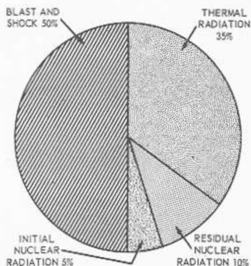
5.166 Figure 14-1.—A typical nuclear energy distribution graph.
