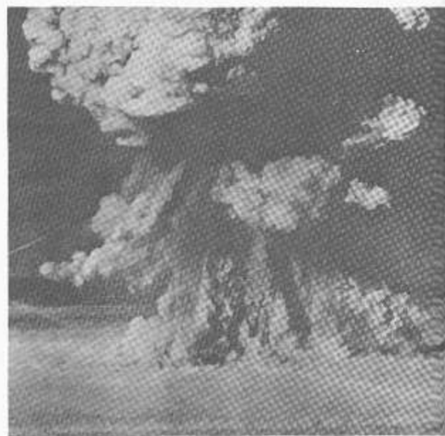
Figure 14-5.—Formation of dirt cloud in surface burst.
