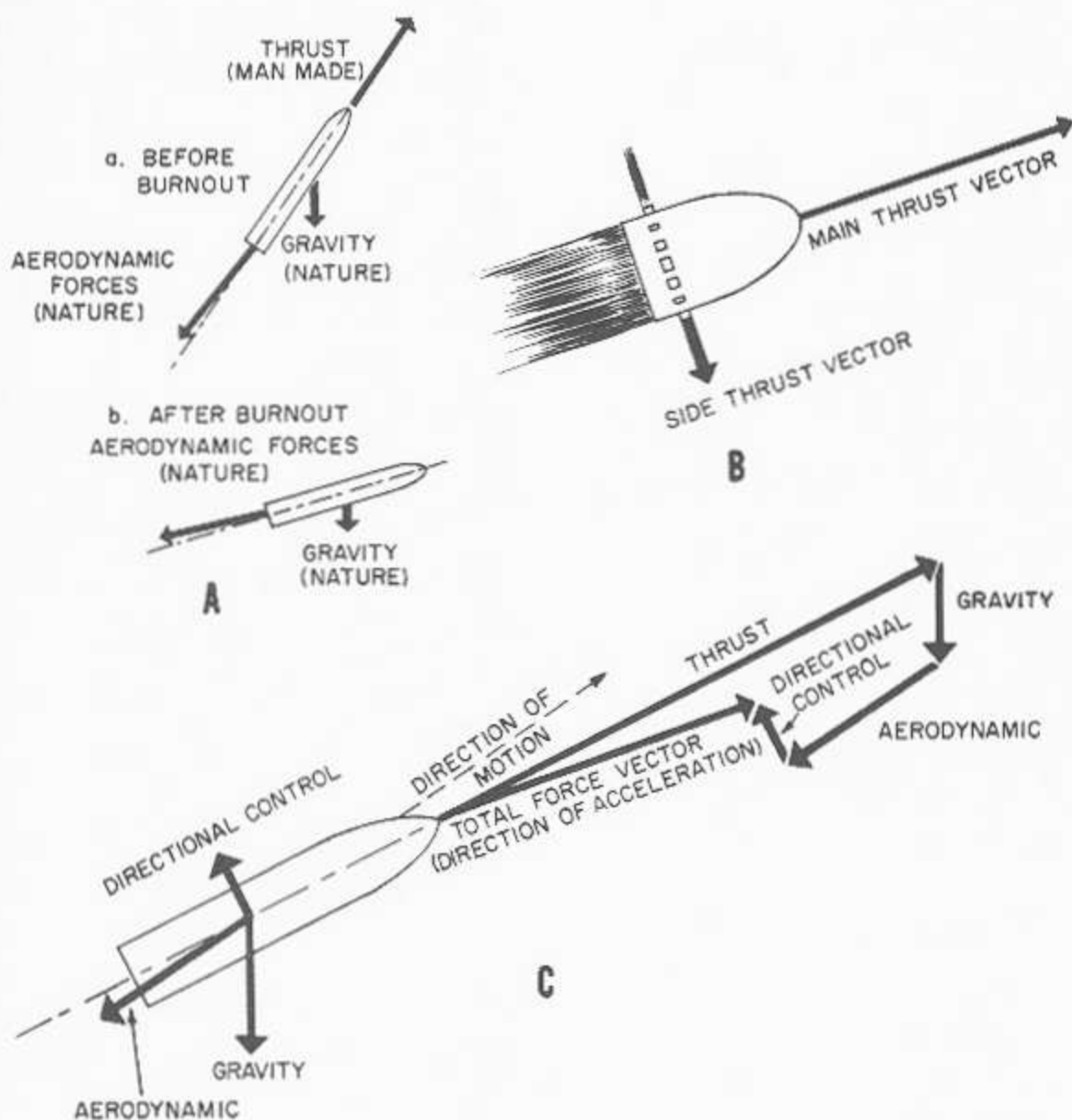
Figure 2-19.—Vector control: A. Before and after burnout; B. Thrust vectors; C. Total force vector.
