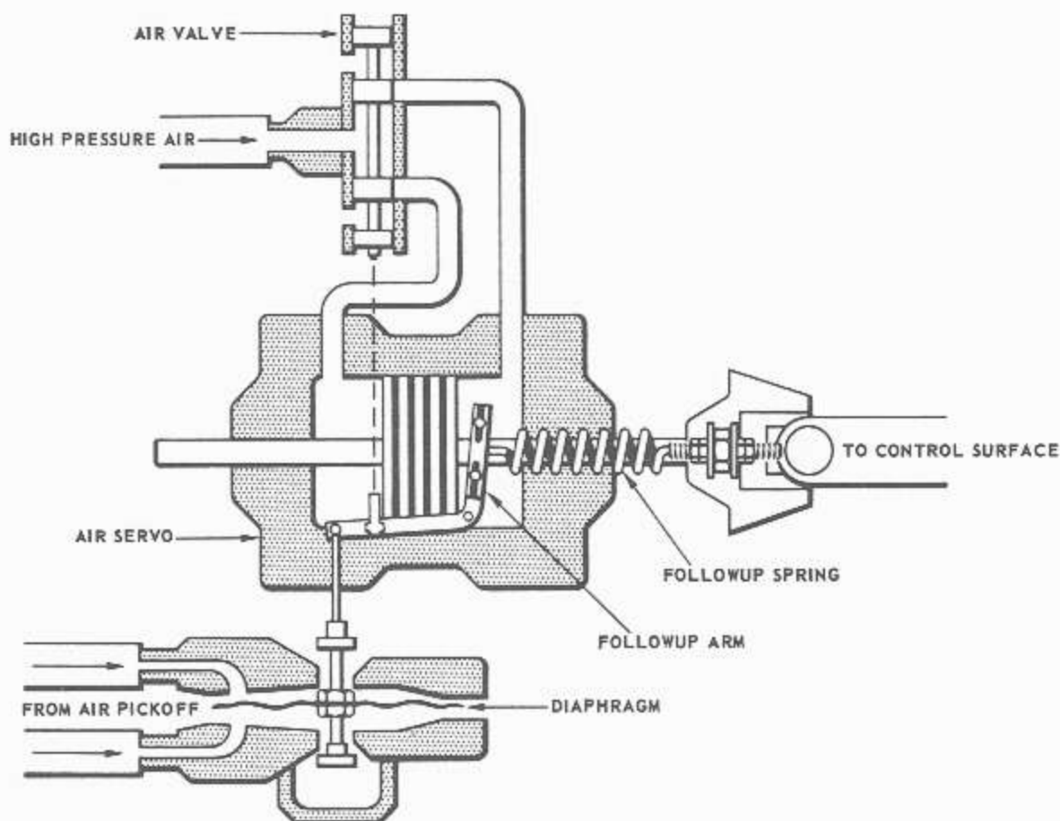
Figure 5-37.—Air relay with mechanical followup.
