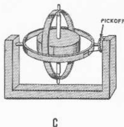
Figure 5-24.—Potentiometers: A. Wire wound potentiometer; B. Helipot; C. Potentiometer pickoff used with a free gyro.
