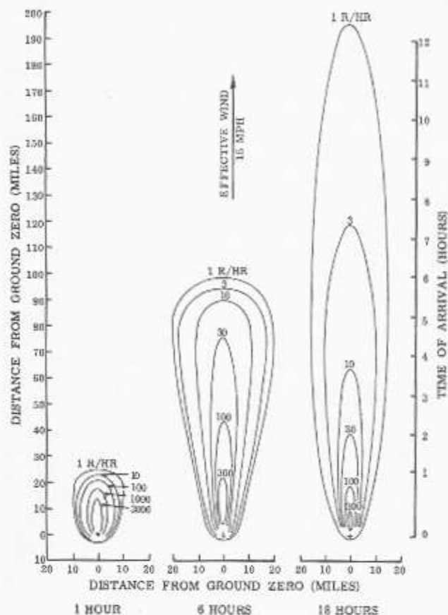
Figure 14-20.—Dose-rate contours from early fallout at 1, 6, and 18 hours after a surface burst with 1-megaton fission yield (15 mph effective wind speed).
