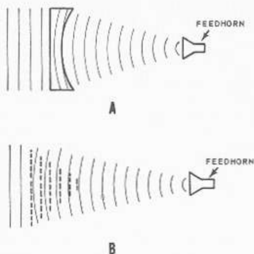
Figure 8-7.—Antenna lenses: A. Waveguide (acceleration) type microwave lens; B. Metal strip (delay) type microwave lens.
