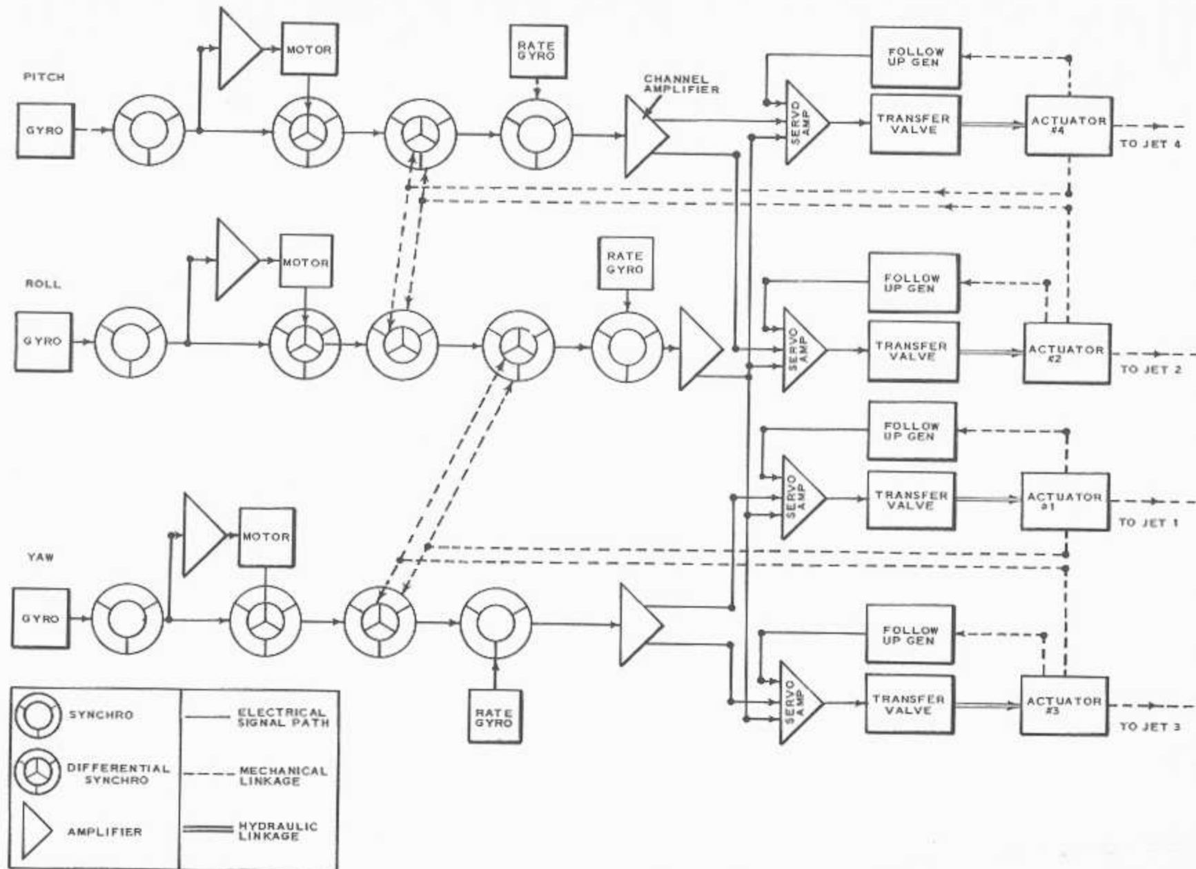
Figure 5-39.—Electrical interconnection of channels in hydraulic-electric control system.
