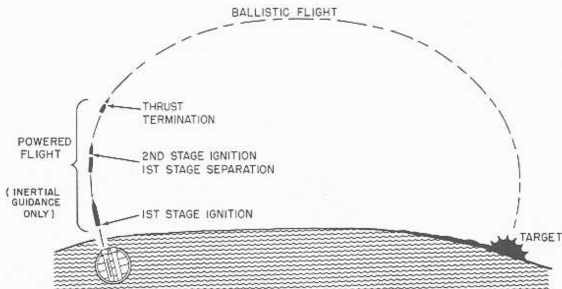
Figure 11-14.—Polaris trajectory (not to scale.)
