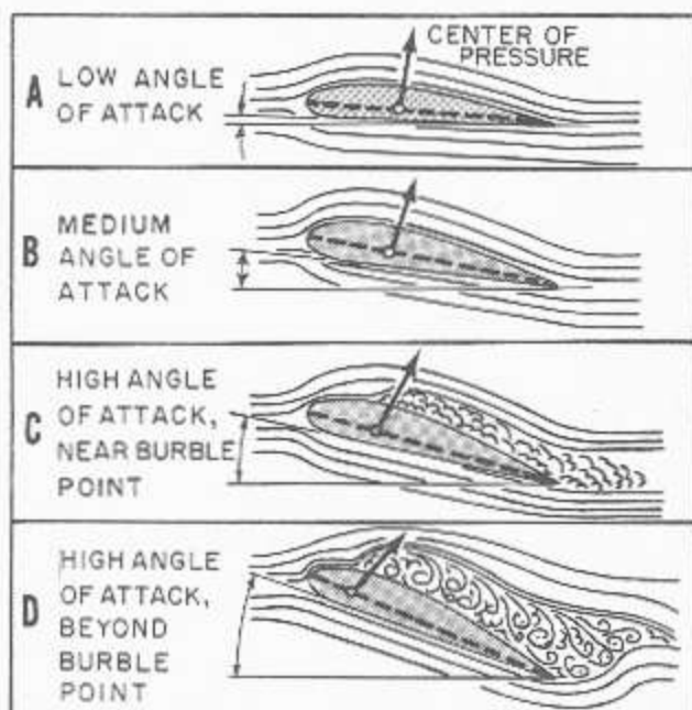
33.24 Figure 2-9.—Effect of angle of attack on center of pressure and air flow.
