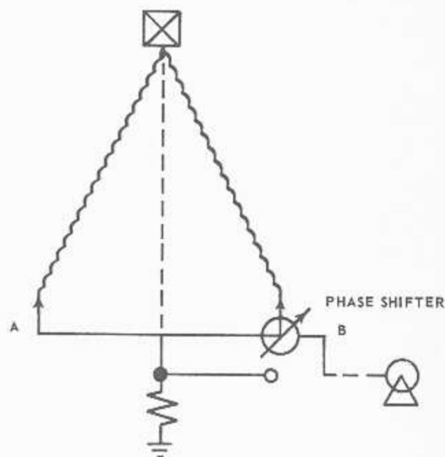
Figure 9-17.—Interferometer with phase shifter on antenna B.
