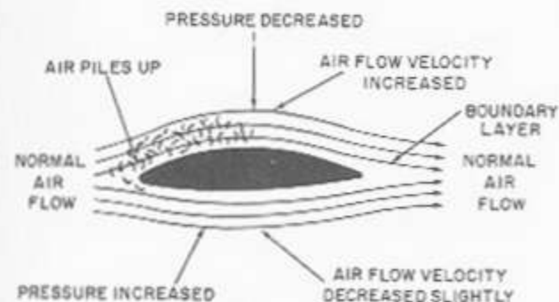
Figure 2-5.—Air flow over a wing section.
