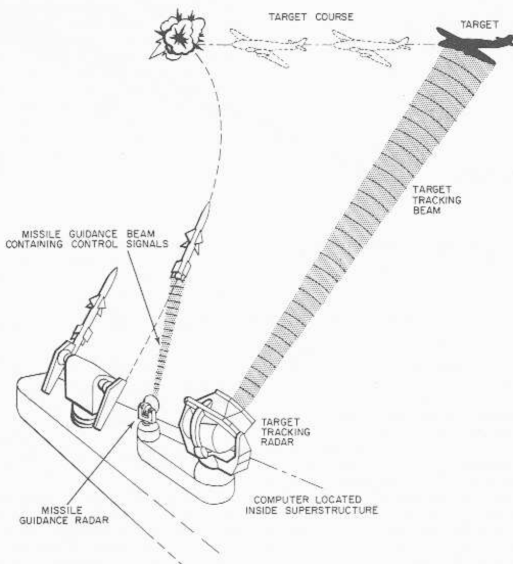
Figure 6-7.—Modified beam-rider guidance.
