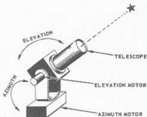
Figure 10-16.—Automatic sextant.
