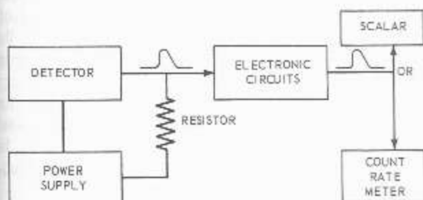
Figure 12-11.—Basic radiac circuit.
