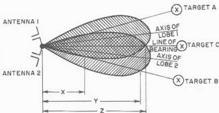
Figure 8-9.—Double-lobe system, showing relation between axis of intersection and target bearing.
