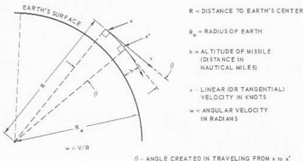
Figure 10-11.—Applying angular velocity to platform leveling.
