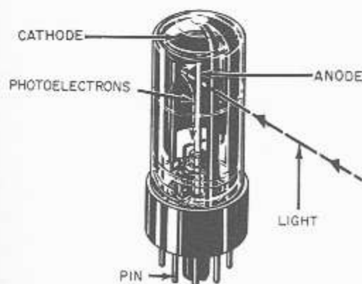
Figure 6-2.—A photoelectric cell.
