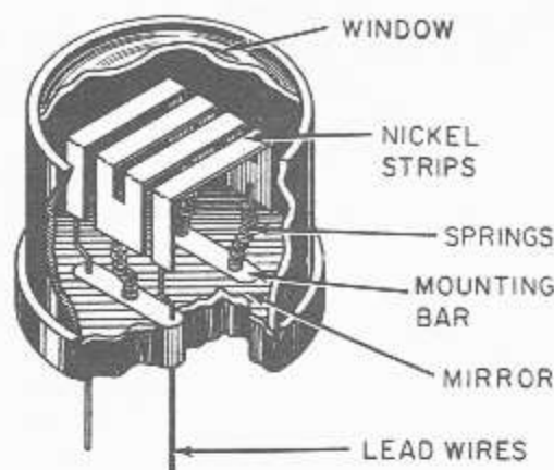
Figure 9-7.—A simple modern bolometer.
