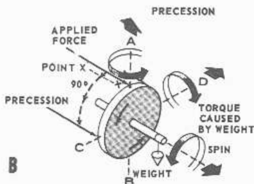
Figure 5-15.—Gyroscopic precession: A. Application of force; B. Direction of precession.
