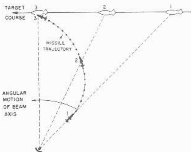
Figure 8-20.—Beam-rider missile following line of sight (LOS) course, increases lateral acceleration as it nears target.
