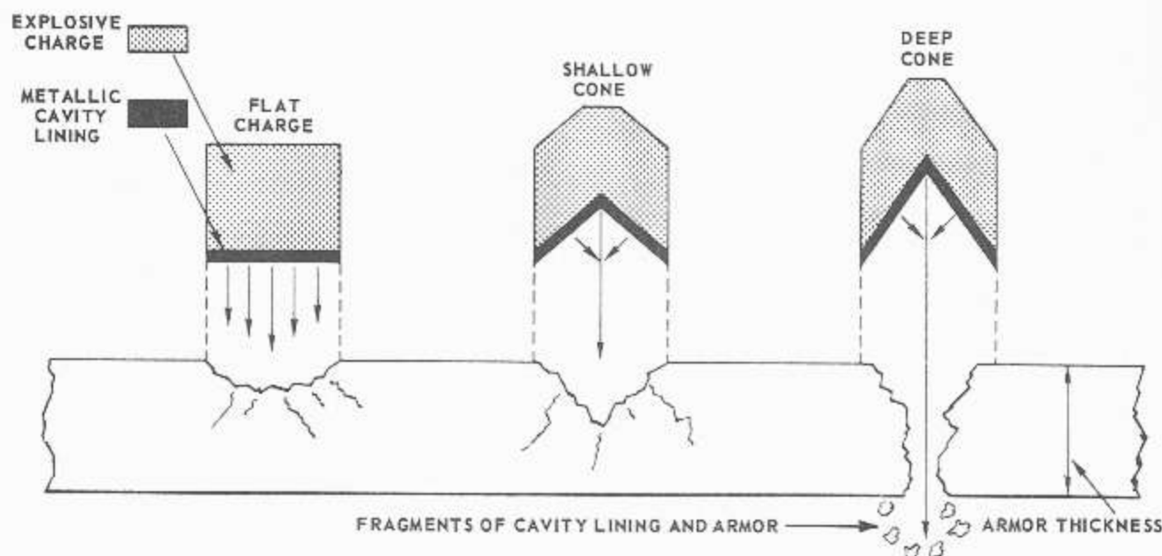
Figure 3-7.—Penetration effectiveness of various shaped charges.
