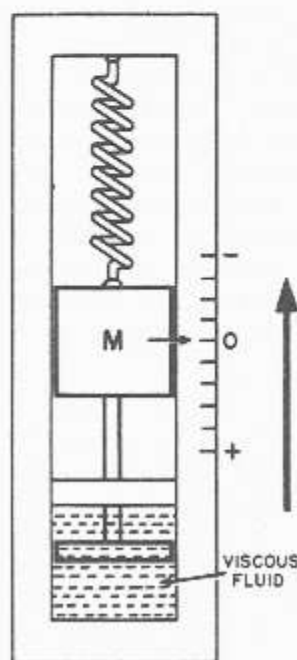
Figure 6-10.—Liquid-damped system.
