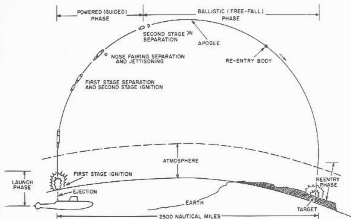
Figure 2-24.—Typical trajectory of an ICBM (Polaris).
