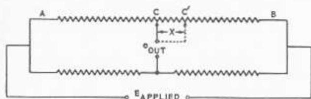
Figure 5-23.—Principle of a potentiometer pickoff.
