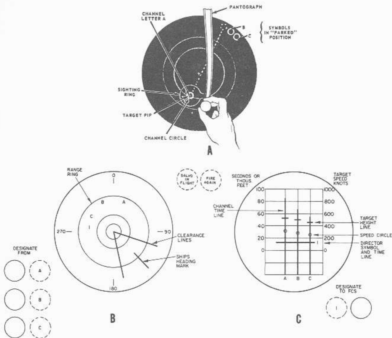
Figure 8-18.—Target information displayed on weapon console scopes: A. Target tracking console display; B. Weapon direction equipment console plan plot display; C. Multipurpose plot.
