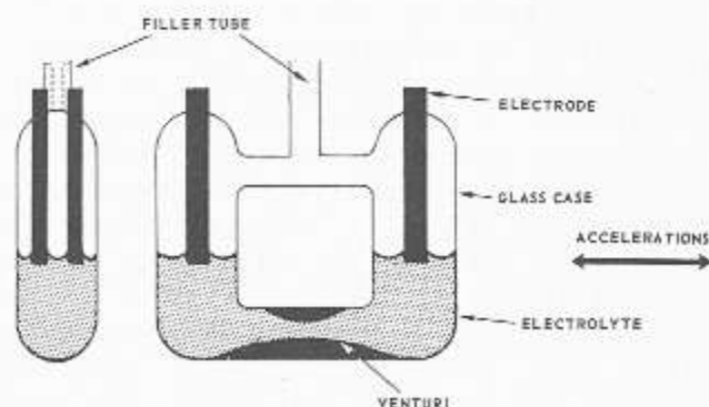
Figure 6-12.—Manometer accelerometer with venturi damper.
