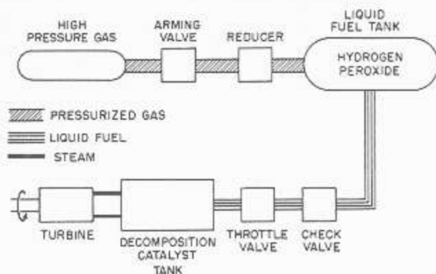
144.28 Figure 5-5.—Basic liquid-propellant auxiliary power supply.
