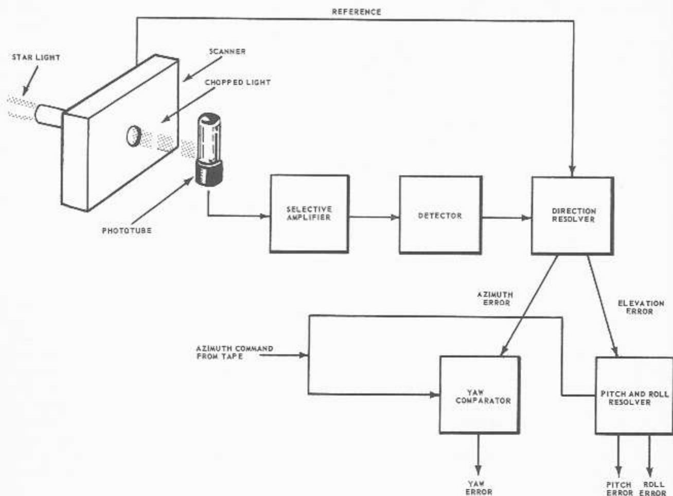
Figure 10-18.—Stellar error-detection circuit.
