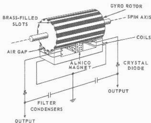
Figure 5-21. Internally operated reluctance pickoff.
