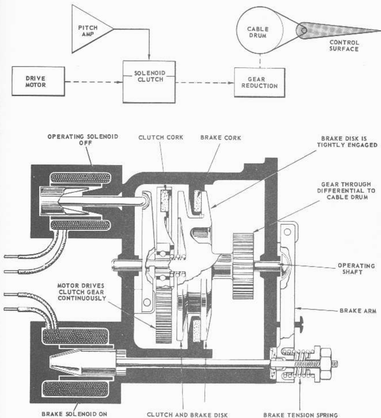
Figure 5-42.—Control system using constant speed actuator motor.
