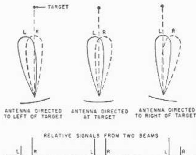
Figure 8-12.—Lobe switching.
