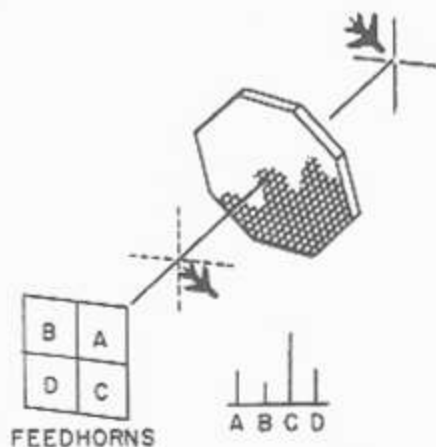
Figure 8-13.—Monopulse technique of radar scanning.
