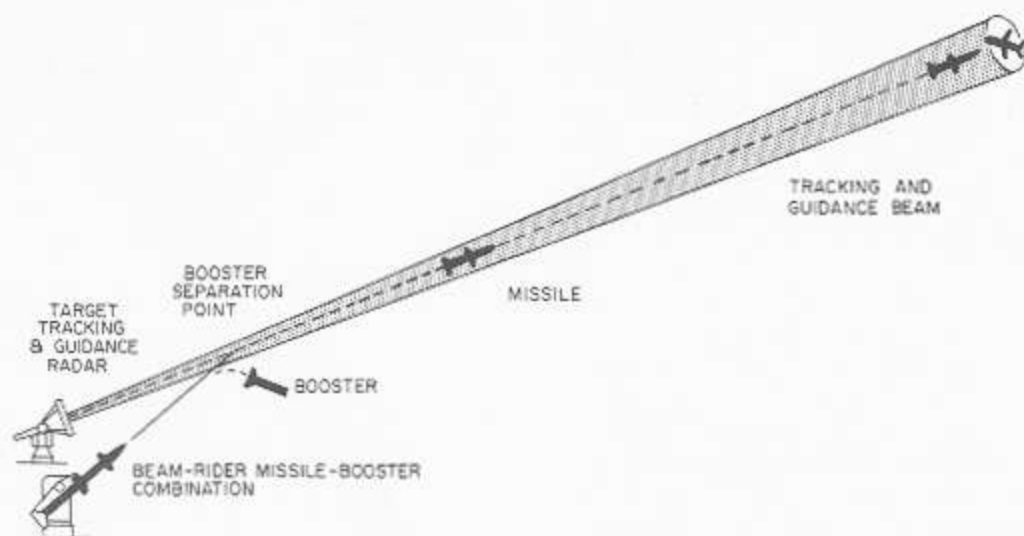
Figure 6-6.—Simple beam-rider guidance system.
