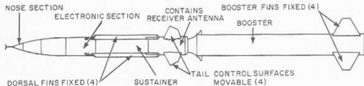
Figure 8-8.—View of beam-rider missile, showing location of control surfaces and receiver antennas.
