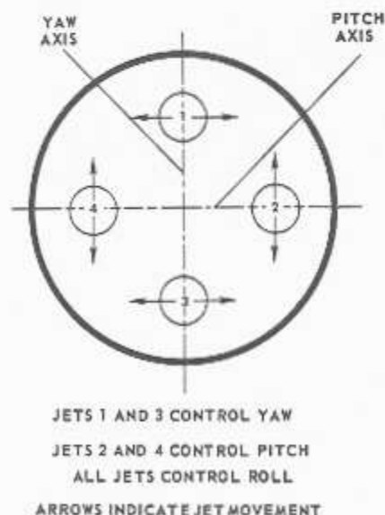
Figure 5-2.—Control by four jets (aft view of missile).
