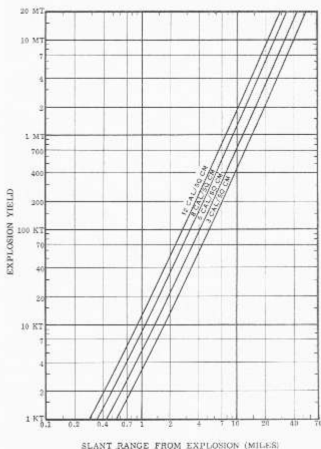
Figure 14-17.—Slant ranges for specified exposures as function of energy yield of the explosion.
