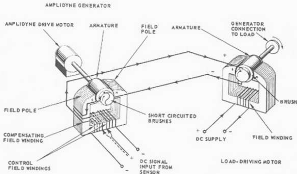
Figure 5-33.—Amplidyne controller.
