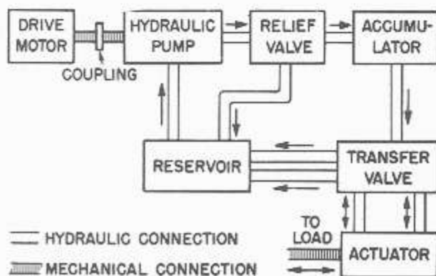
33.182 Figure 5-34.—Basic hydraulic controller.
