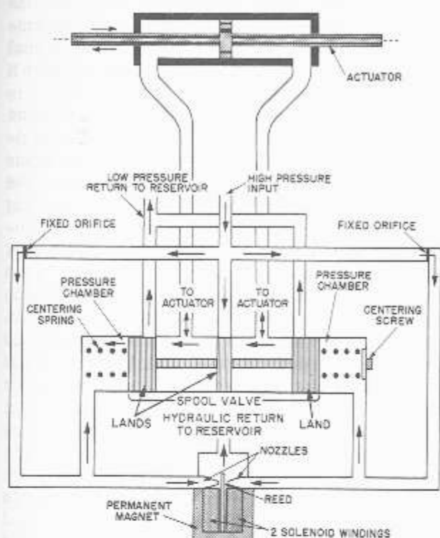
Figure 5-31.—Servovalve.
