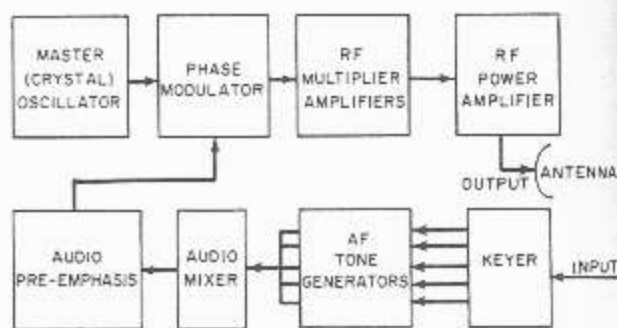
Figure 7-2.—Phase modulated radio command transmitter.
