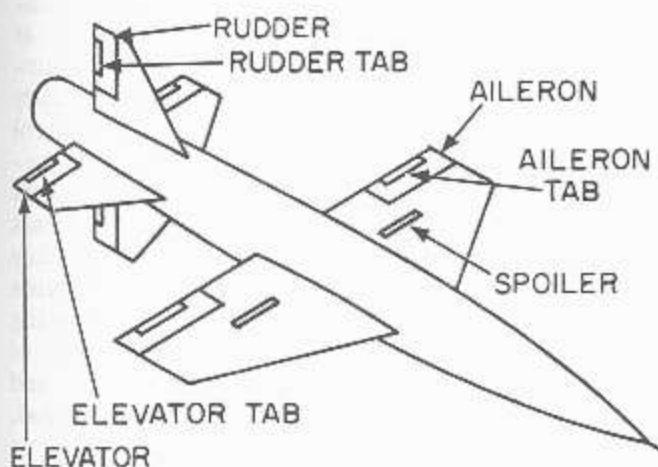
Figure 2-17.—Control devices on conventional type missiles.
