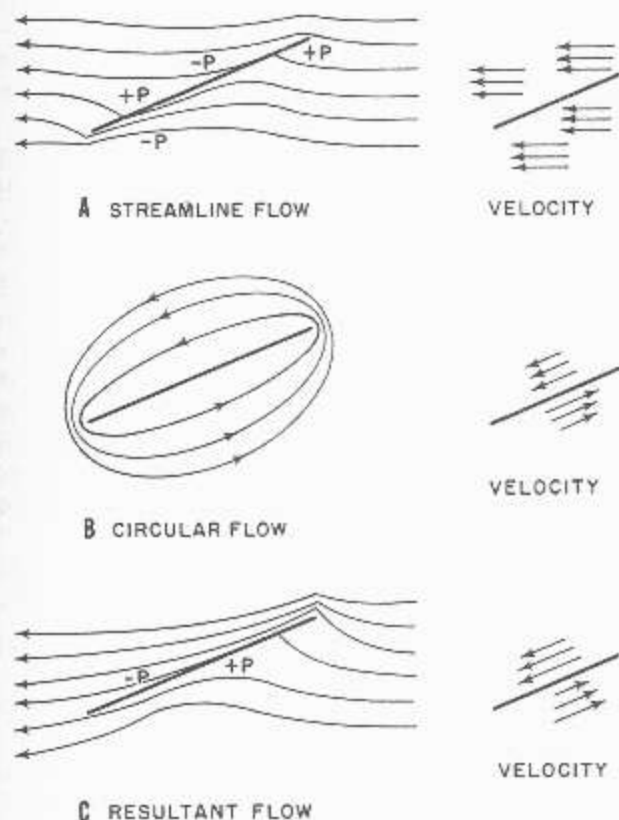
144.11 Figure 2-23.—Flow of water about an inclined plane: A. Streamline flow; B. Circular flow; C. Resultant flow.
