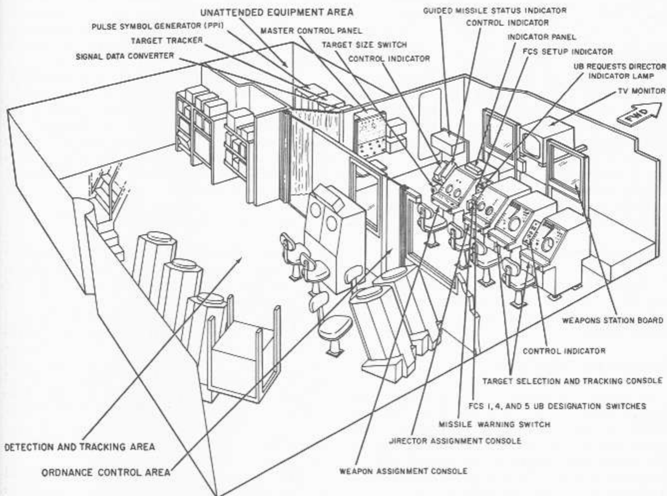
Figure 11-11.—Weapons control station.
