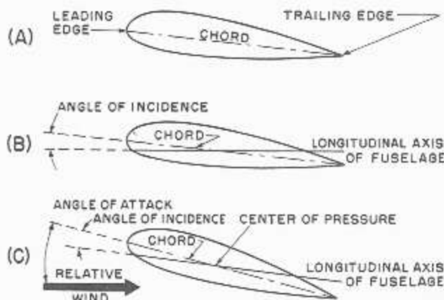
33.24 Figure 2-8.—Standard nomenclature applied to airfoils.
