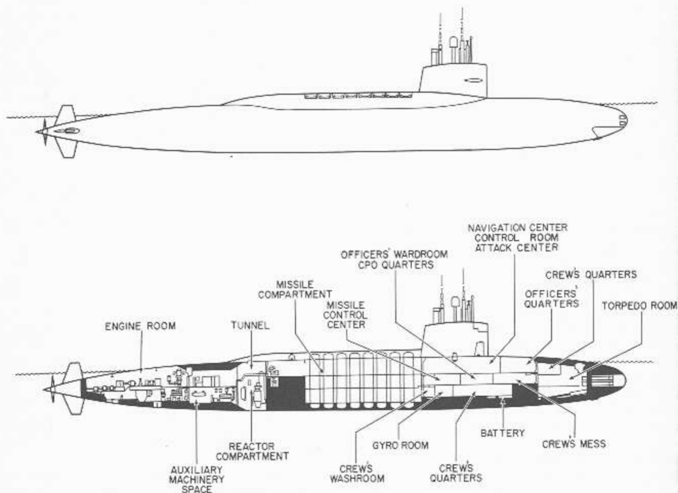
Figure 11-13.—SSB class submarine.
