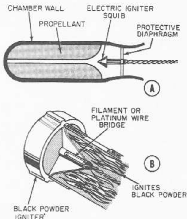
Figure 4-7.—Types of igniters: A. Electric igniter squib type; B. Black powder charge igniter.
