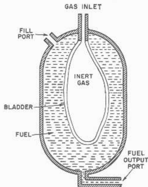
144.29 Figure 5-6.—Fuel tank in liquid-propellant auxiliary power system.
