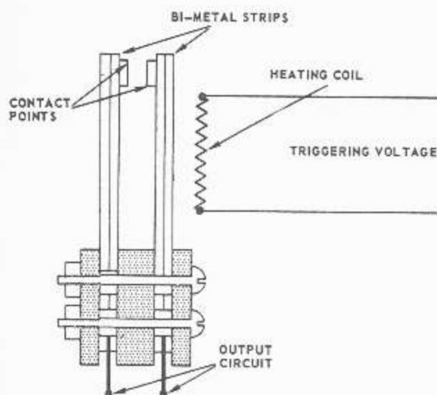
Figure 5-12.—Thermal delay tube.
