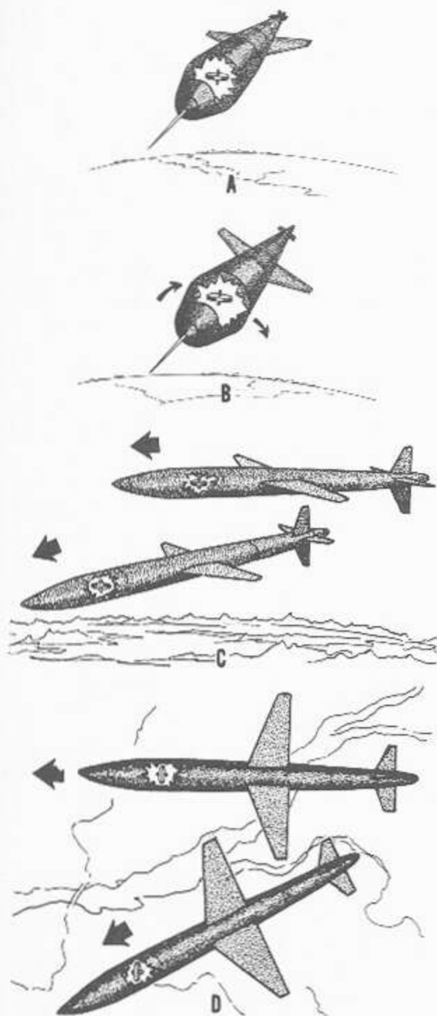
Figure 5-18.—Free gyro behavior in missiles: A. Missile horizontal—gyro stable in space; B. Missile rolls—gyro remains stable; C. Mis- sile pitches—gyro remains stable; D. Missile yaws—gyro remains stable.
