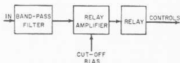
Figure 7-4.—Selector channel with band-pass filter.
