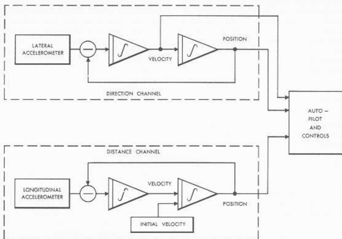
Figure 10-5.—Simple inertial guidance system.
