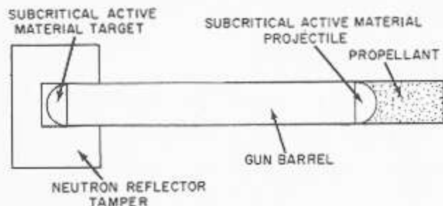
Figure 13-1.—Idealized gun type weapon.
