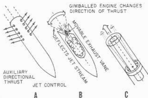
Figure 2-18.—Jet control of flight attitude.
