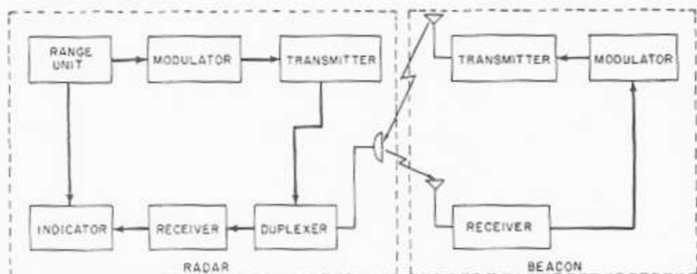
Figure 7-7.—Radar beacon system in missile guidance.
