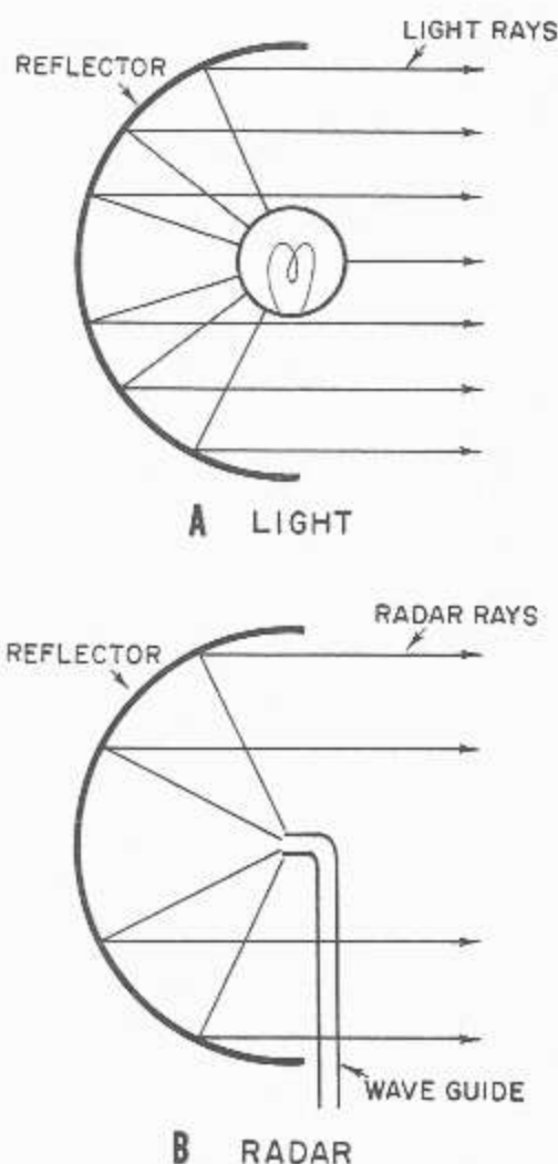
Figure 8-4.—Radiation of light and radar waves as affected by a reflector.
