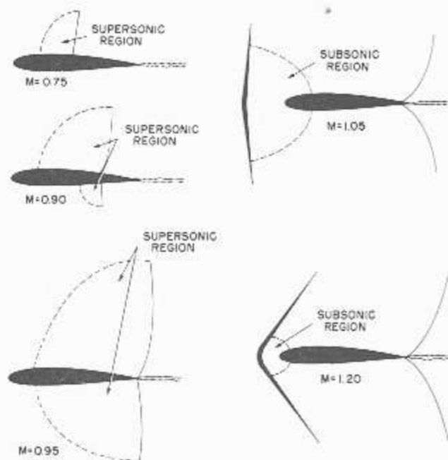
Figure 2-15.—Shock waves at various speeds of airfoils.
