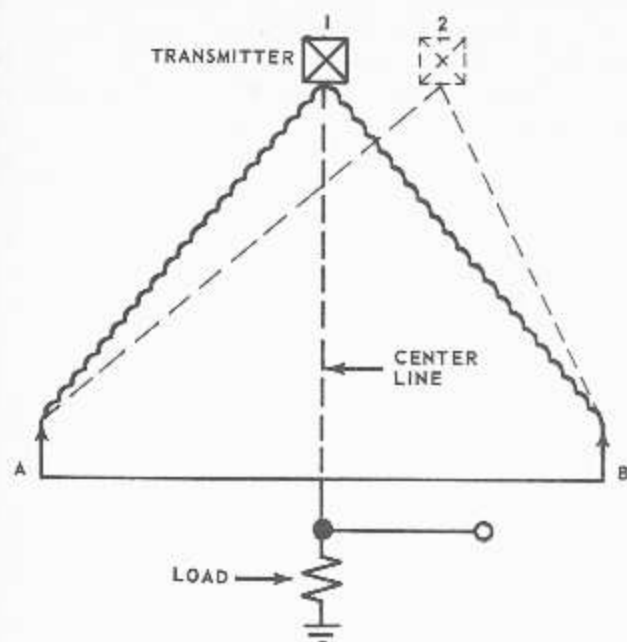
Figure 9-16.—Interferometer principle.
