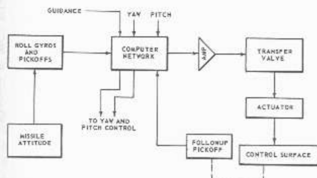
Figure 5-38.—Hydraulic-electric channel for roll control.
