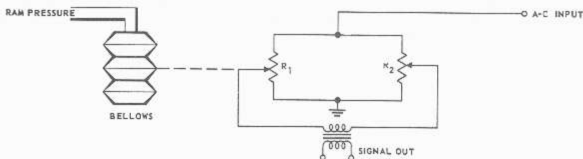
Figure 5-20.—Airspeed transducer.
