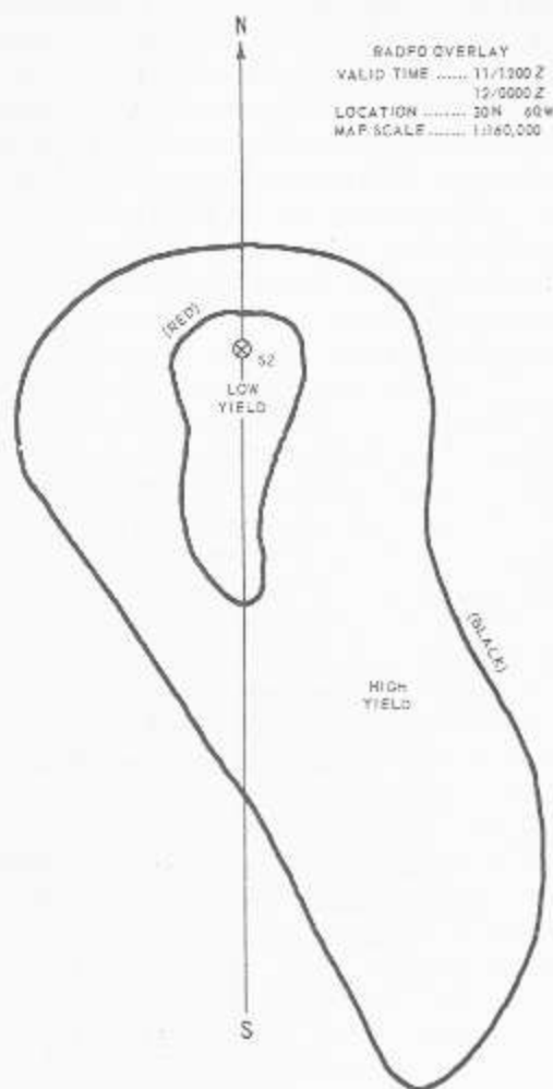
Figure 14-22.—Example of fallout plot drawn with RAD FO overlay upon receipt of prediction or warning message.
