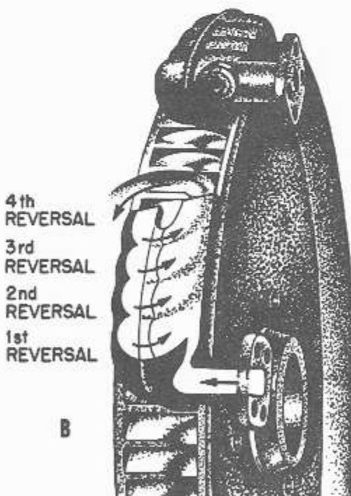
33.45:46 Figure 5-4.—Turbines used in auxiliary power supply (APS): A. Impulse turbine; B. Terry turbine.
