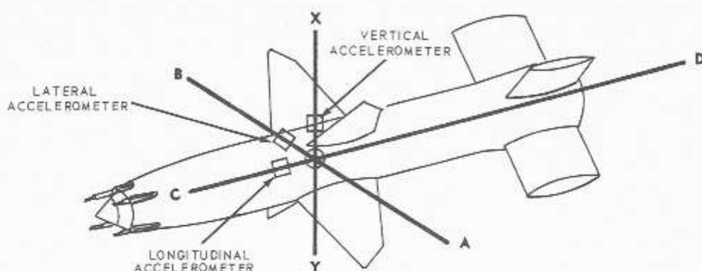
Figure 6-9.—Accelerometers in guided missiles.
