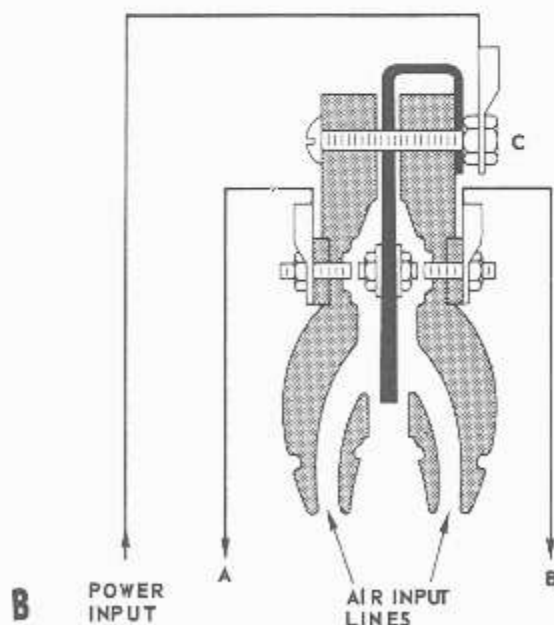
Figure 5-32.—Some types of relays in missiles: A. Low current relay; B. Air-actuated relay.
